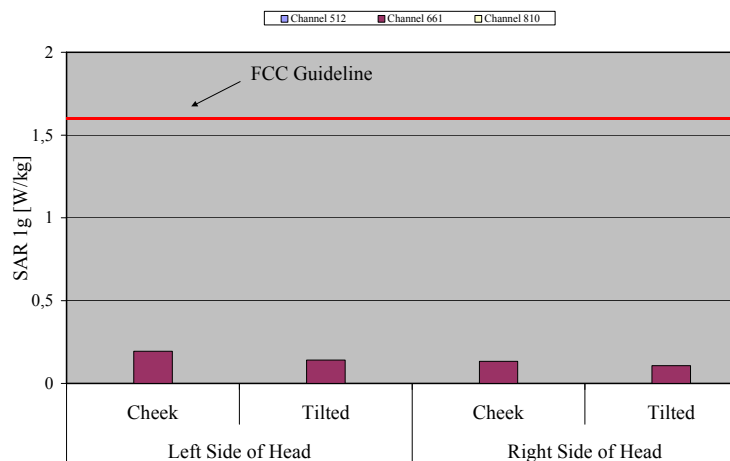
Fig. 7: The measured head phantom SAR values for the Alcatel One Touch 556 for PCS 1900 in comparison to the FCC exposure limit.
