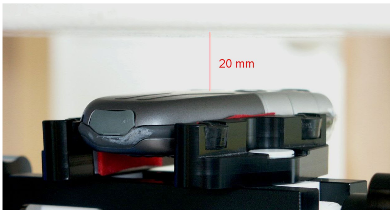
Fig. 17: Body worn configuration, GPRS mode (2 TX slots), antenna towards the phantom.
