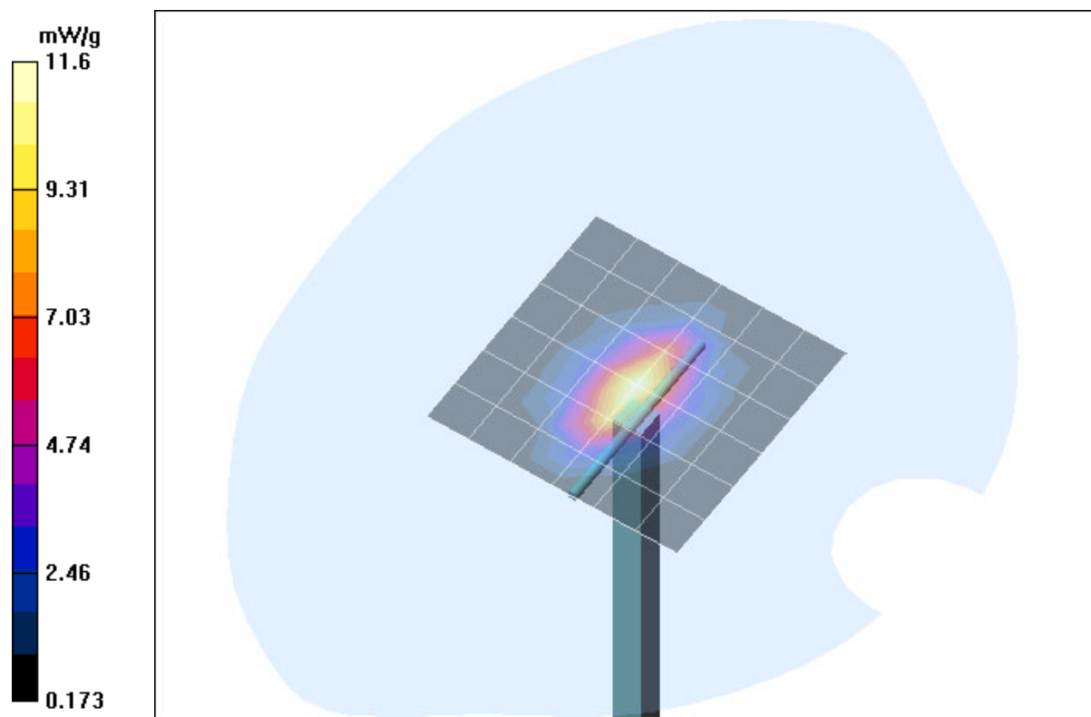
Fig. 9: Validation measurement 1900 MHz Head (July 14, 2004), coarse grid. Ambient Temperature: 21.1° C, Liquid Temperature: 20.6 C.
