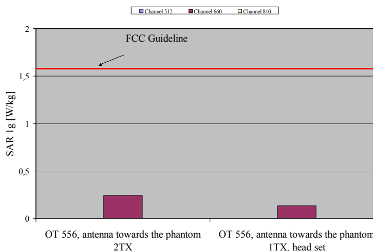
Fig. 7: The measured head phantom SAR values for the Alcatel One Touch 556 for PCS 1900 in comparison to the FCC exposure limit.
