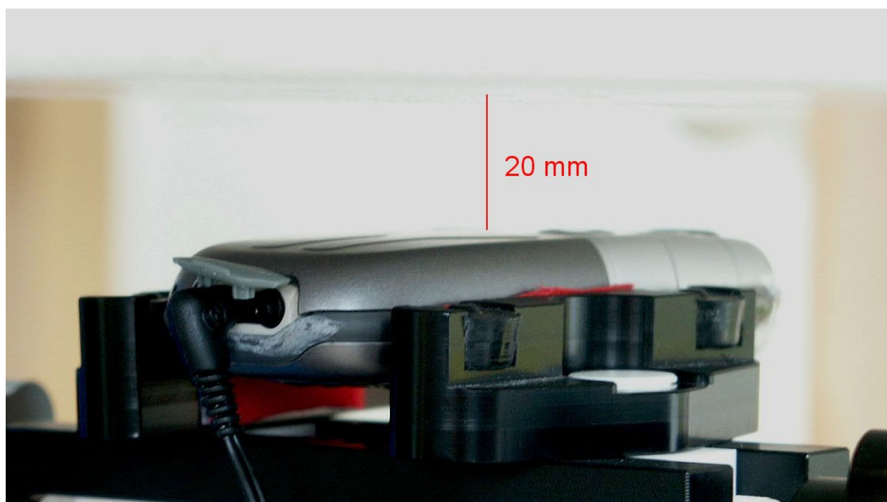
Fig. 18: Body worn configuration, GSM mode (1 TX slot) with headset, antenna towards the phantom.
