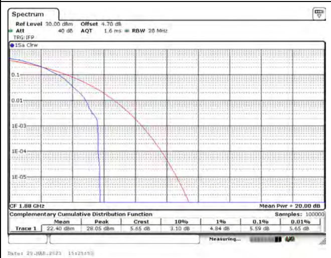
LTE Band 2_CH18900_1.4M_64-QAM_1RB0
