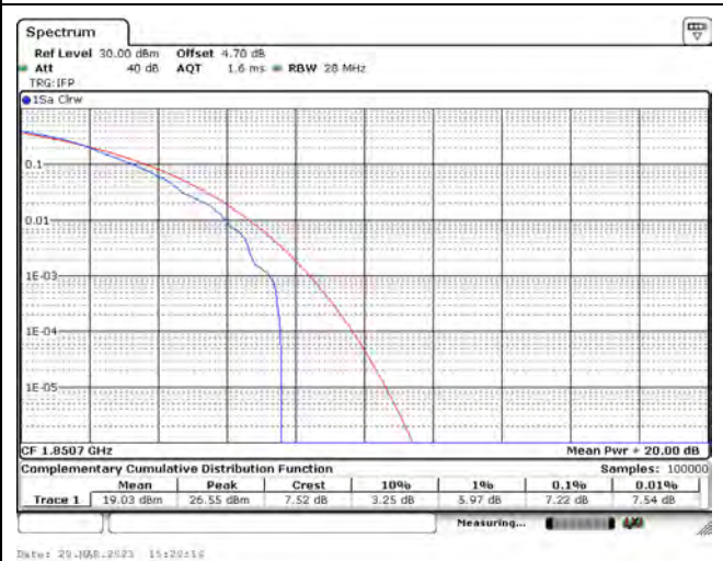
LTE Band 2_CH18607_1.4M_256-QAM_1RB0
