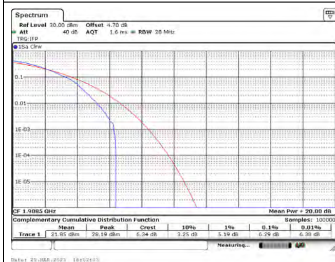
LTE Band 2_CH19185_3M_64-QAM_1RB14
