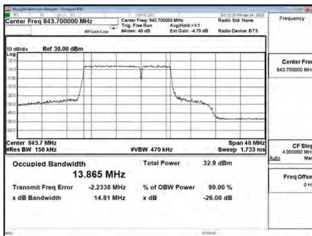
LTE CA Band 5B_256-QAM_CH20500+CH20572_10M+5M_50RB0+25RB0
