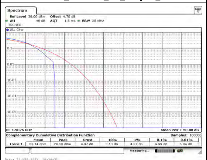
LTE Band 2_CH19175_5M_16-QAM_1RB24
