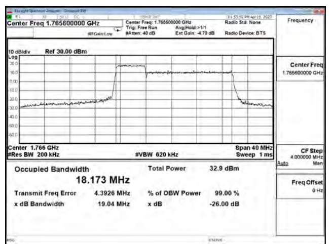
LTE CA Band 66B_16-QAM_CH132504+CH132597_5M+15M_25RB0+75RB0
