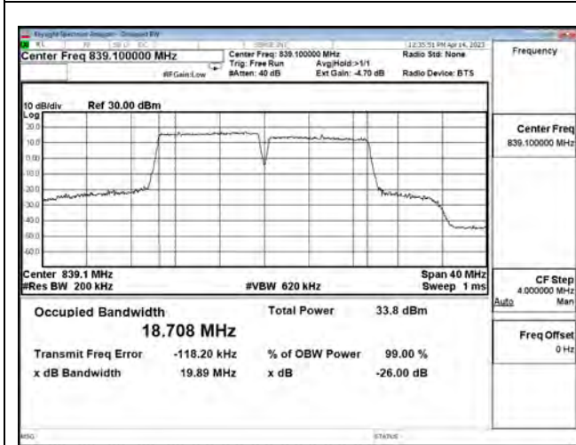
LTE CA Band 5B_64-QAM_CH20501+CH20600_10M+10M_50RB0+50RB0
