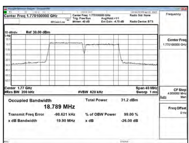
LTE CA Band 66B_256-QAM_CH132523+CH132622_10M+10M_50RB0+50RB0
