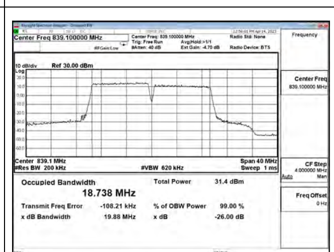
LTE CA Band 5B_256-QAM_CH20501+CH20600_10M+10M_50RB0+50RB0
