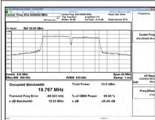
LTE CA Band 5B_64-QAM_CH20450+CH20549_10M+10M_50RB0+50RB0
