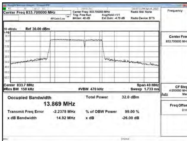
LTE CA Band 5B_64-QAM_CH20550+CH20622_10M+5M_50RB0+25RB0
