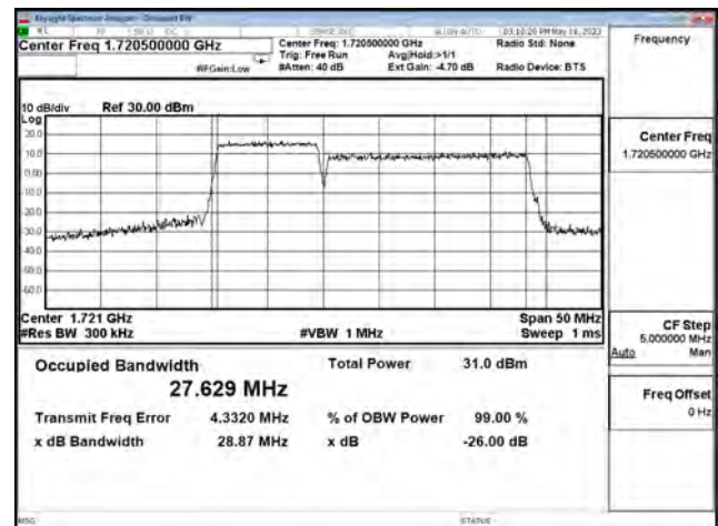
LTE CA Band 66C_16-QAM_CH132428+CH132572_10M+20M_50RB0+100RB0
