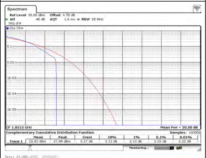
LTE Band 2_CH18615_3M_16-QAM_1RB0
