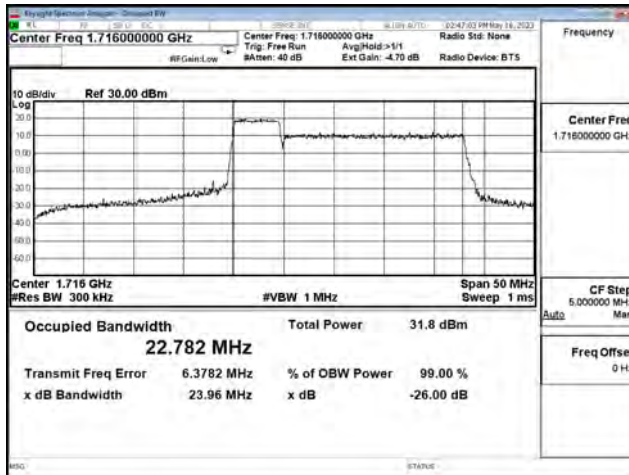
LTE CA Band 66C_QPSK_CH132455+CH132572_5M+20M_25RB0+100RB0
