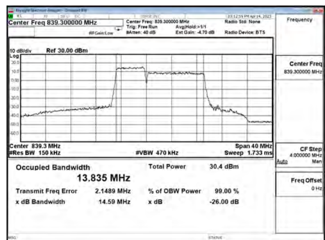
LTE CA Band 5B_256-QAM_CH20528+CH20600_5M+10M_25RB0+50RB0
