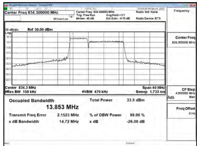
LTE CA Band 5B_16-QAM_CH20428+CH20500_5M+10M_25RB0+50RB0
