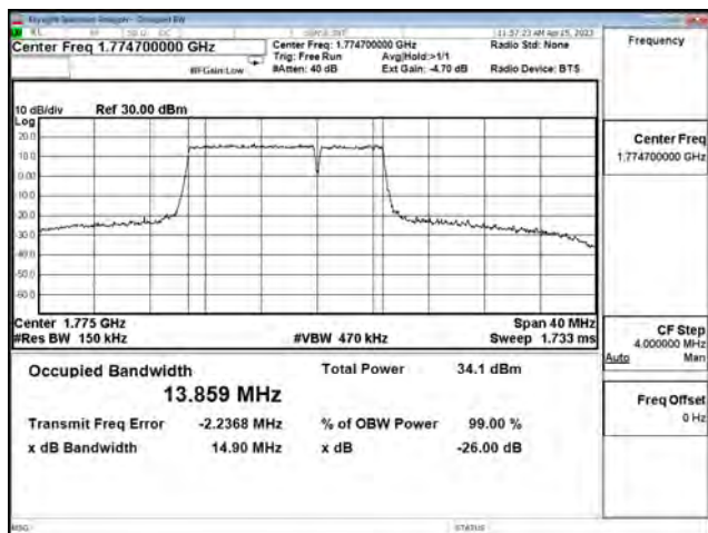
LTE CA Band 66B_16-QAM_CH132397+CH132469_10M+5M_50RB0+25RB0
