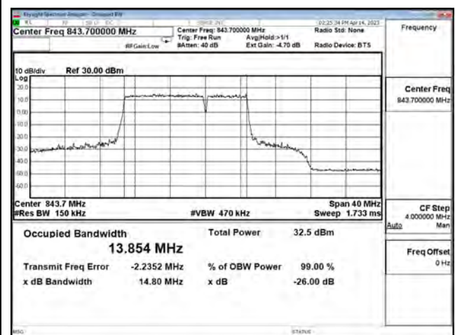
LTE CA Band 5B_16-QAM_CH20550+CH20622_10M+5M_50RB0+25RB0
