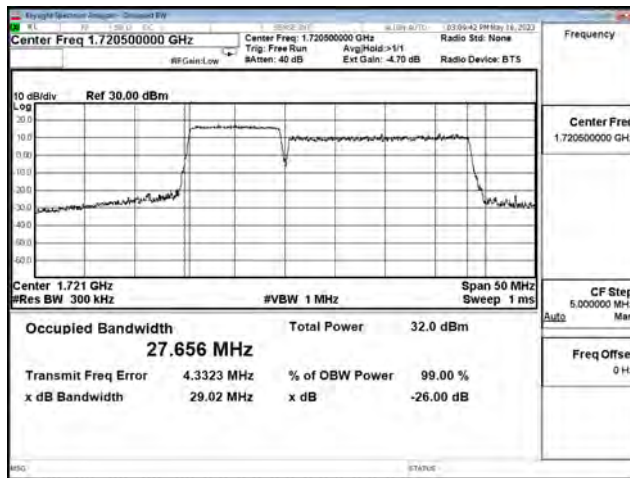
LTE CA Band 66C_QPSK_CH132428+CH132572_10M+20M_50RB0+100RB0
