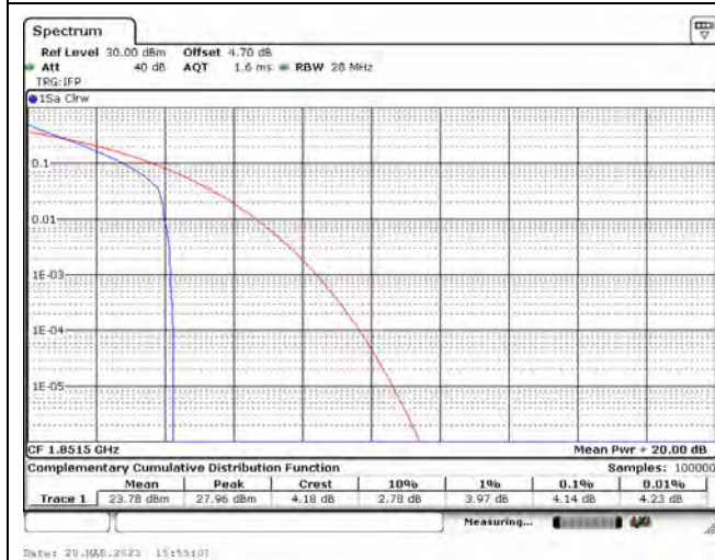
LTE Band 2_CH18615_3M_QPSK_1RB0
