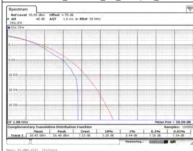
LTE Band 2_CH18900_3M_256-QAM_1RB0
