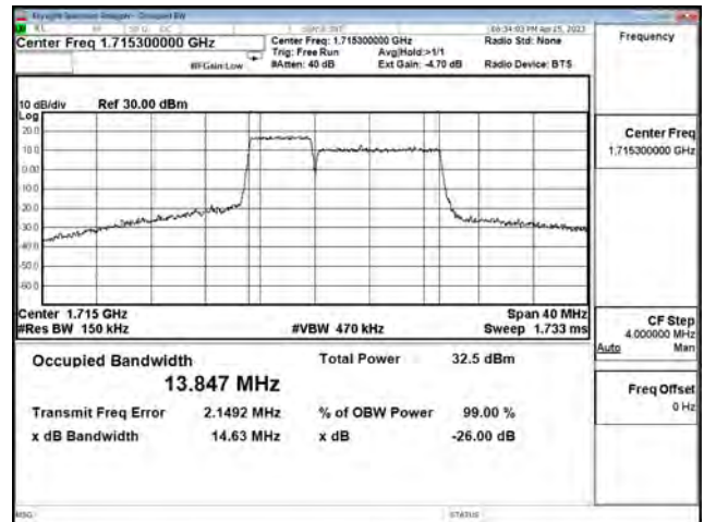
LTE CA Band 66B_16-QAM_CH132550+CH132662_5M+10M_25RB0+50RB0
