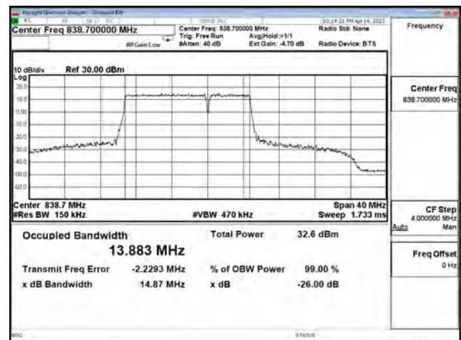
LTE CA Band 5B_256-QAM_CH20450+CH20522_10M+5M_50RB0+25RB0
