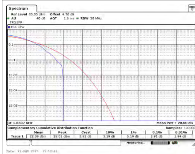
LTE Band 2_CH18607_1.4M_64-QAM_1RB0
