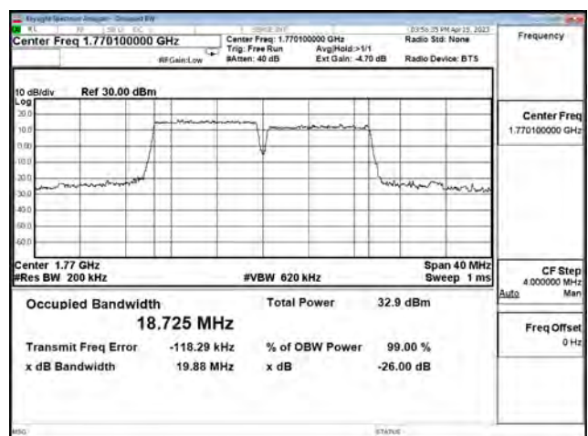
LTE CA Band 66B_16-QAM_CH132523+CH132622_10M+10M_50RB0+50RB0
