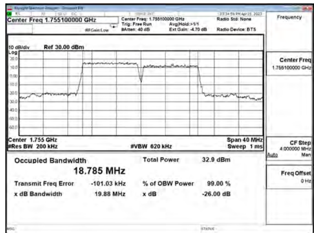
LTE CA Band 66B_16-QAM_CH132022+CH132121_10M+10M_50RB0+50RB0
