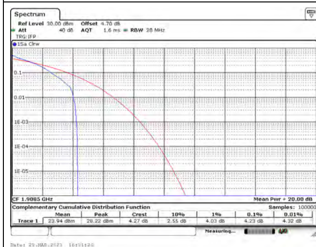
LTE Band 2_CH19185_3M_QPSK_1RB14
