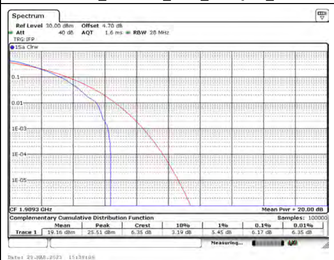
LTE Band 2_CH19193_1.4M_256-QAM_1RB5
