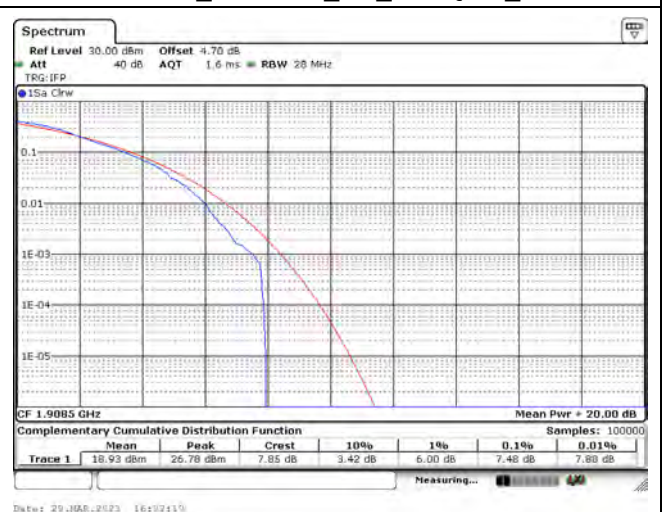
LTE Band 2_CH19185_3M_256-QAM_1RB14
