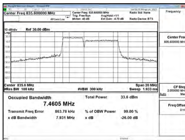
LTE CA Band 5B_16-QAM_CH20501+CH20540_3M+5M_15RB0+25RB0
