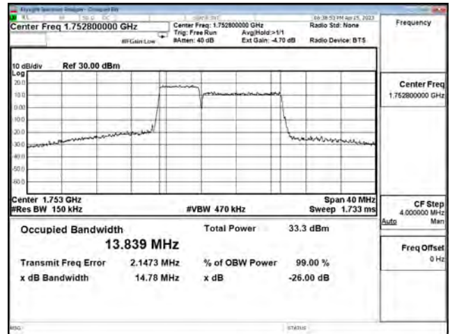
LTE CA Band 66B_16-QAM_CH132000+CH132072_5M+10M_25RB0+50RB0
