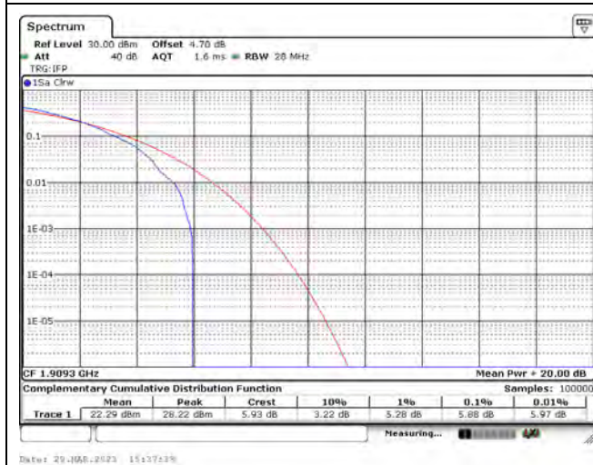
LTE Band 2_CH19193_1.4M_64-QAM_1RB5
