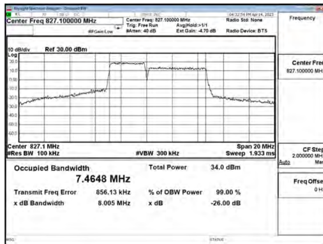
LTE CA Band 5B_QPSK_CH20586+CH20625_3M+5M_15RB0+25RB0
