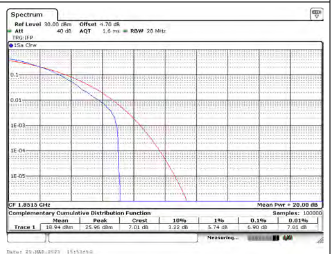
LTE Band 2_CH18615_3M_256-QAM_1RB0
