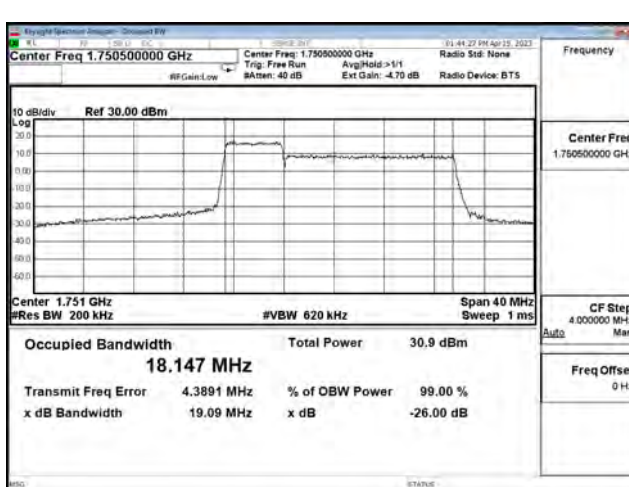
LTE CA Band 66B_256-QAM_CH132353+CH132446_5M+15M_25RB0+75RB0
