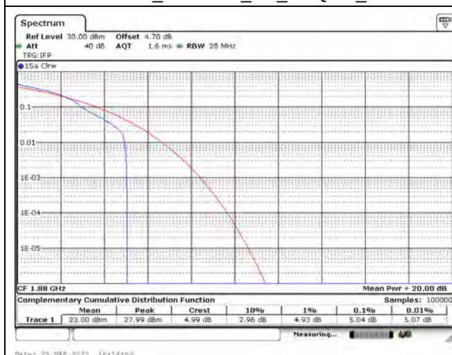
LTE Band 2_CH18900_5M_16-QAM_1RB0
