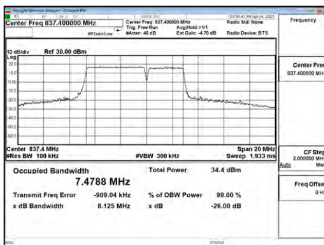
LTE CA Band 5B_16-QAM_CH20510+CH20549_5M+3M_25RB0+15RB0
