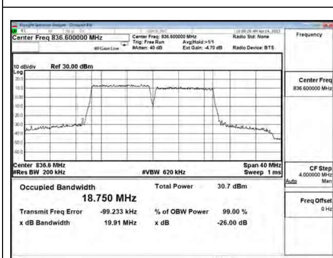
LTE CA Band 5B_256-QAM_CH20476+CH20575_10M+10M_50RB0+50RB0
