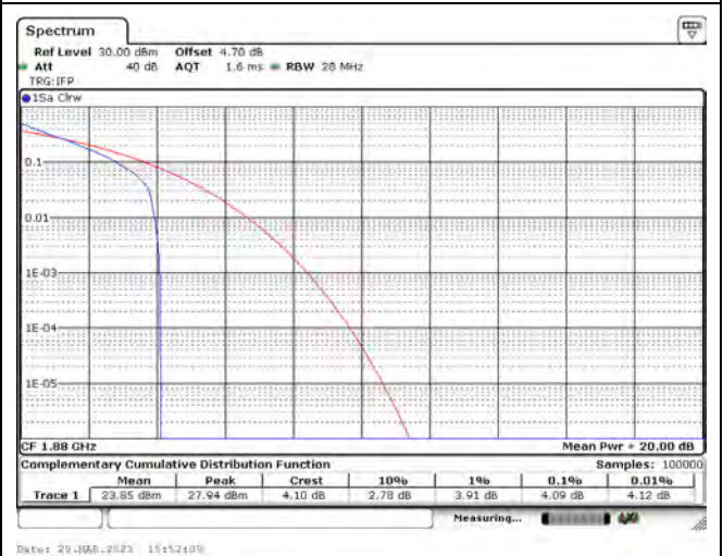
LTE Band 2_CH18900_3M_QPSK_1RB0
