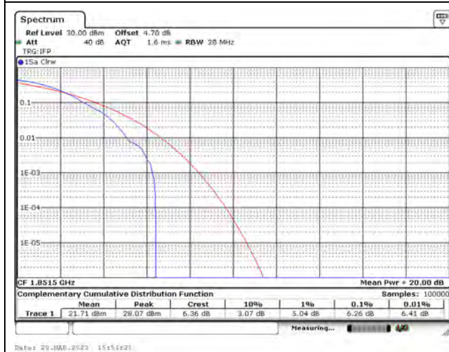
LTE Band 2_CH18615_3M_64-QAM_1RB0
