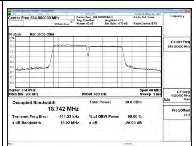
LTE CA Band 5B_256-QAM_CH20450+CH20549_10M+10M_50RB0+50RB0
