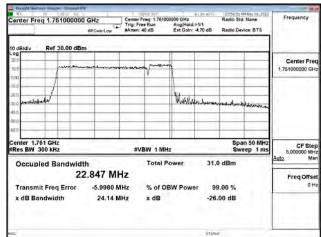
LTE CA Band 66C_256-QAM_CH132072+CH132189_20M+5M_100RB0+25RB0
