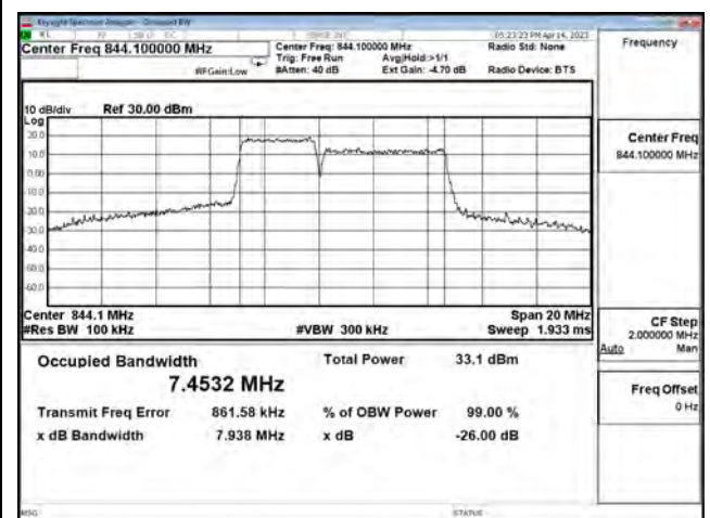
LTE CA Band 5B_16-QAM_CH20586+CH20625_3M+5M_15RB0+25RB0
