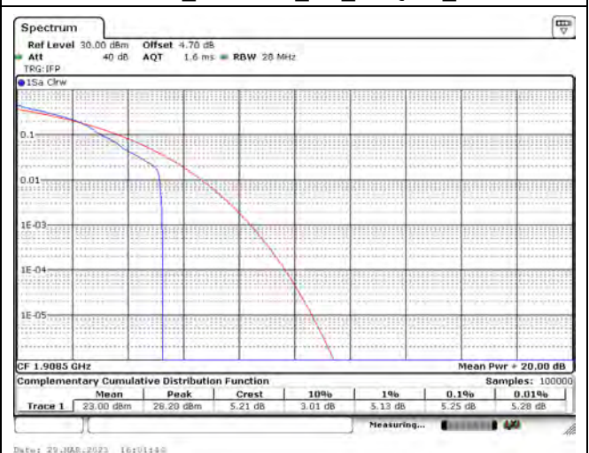
LTE Band 2_CH19185_3M_16-QAM_1RB14
