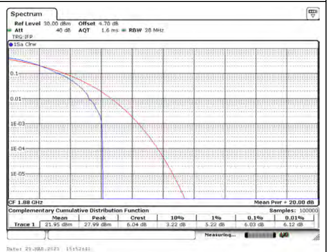
LTE Band 2_CH18900_3M_64-QAM_1RB0
