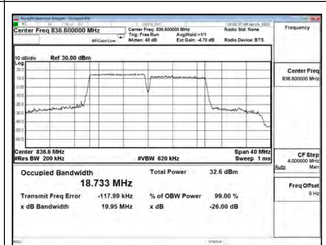
LTE CA Band 5B_64-QAM_CH20476+CH20575_10M+10M_50RB0+50RB0
