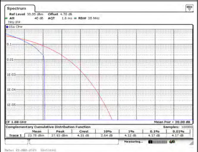
LTE Band 2_CH18900_5M_QPSK_1RB0
