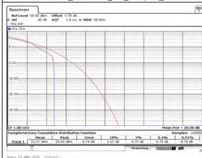
LTE Band 2_CH18900_3M_16-QAM_1RB0
