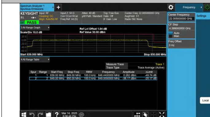
Band5-10MHz-QPSK-20600-50RB#0-PASS
