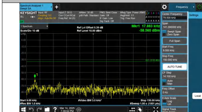
Band5-1.4MHz-QPSK-20643-1RB#0-0.009~0.15-PASS
