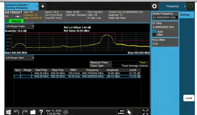
Band5-3MHz-QPSK-20635-1RB#14-PASS
