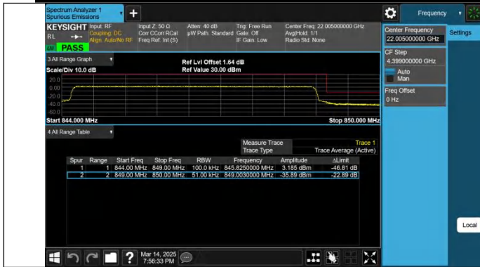
Band5-5MHz-QPSK-20625-25RB#0-PASS
