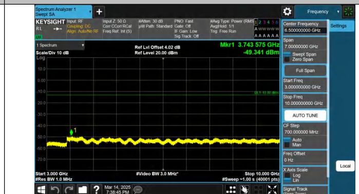
Band5-1.4MHz-QPSK-20525-1RB#5-3000~10000-PASS
