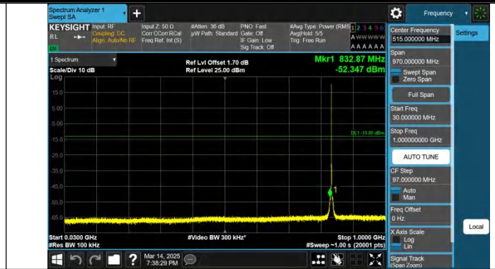
Band5-1.4MHz-QPSK-20525-1RB#5-30~1000-PASS
