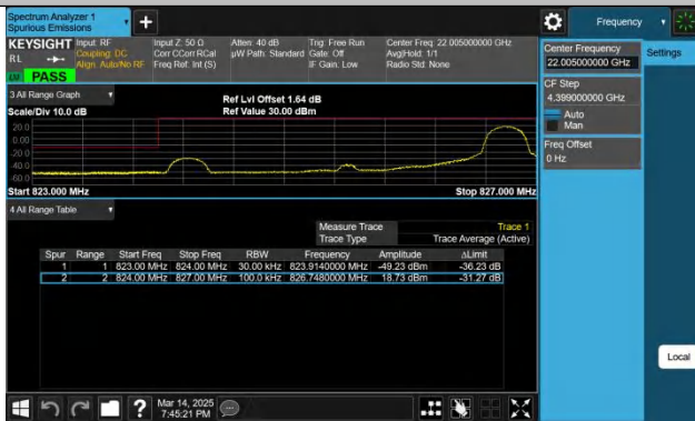
Band5-3MHz-QPSK-20415-1RB#14-PASS
