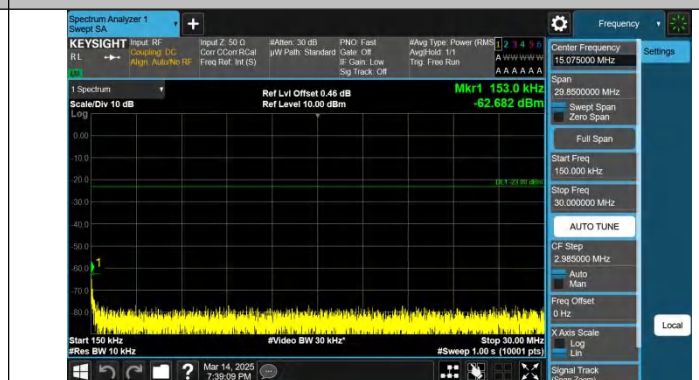
Band5-1.4MHz-QPSK-20643-1RB#0-0.15~30-PASS
