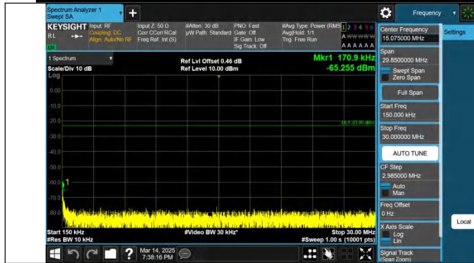
Band5-1.4MHz-QPSK-20525-1RB#5-0.15~30-PASS
