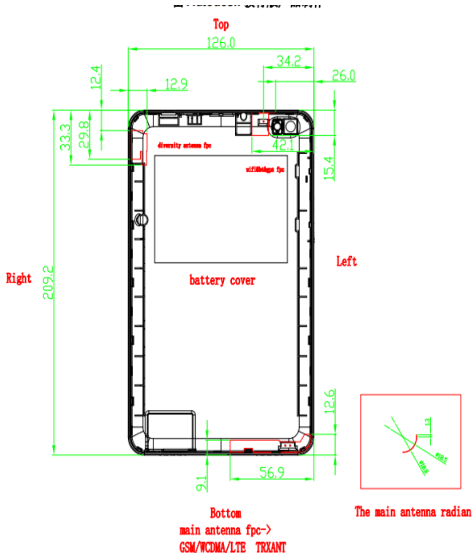
Fig.11.1 EUT Antenna Locations
