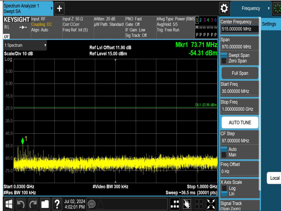
DH5-Ant1-2441-30~1000-PASS
