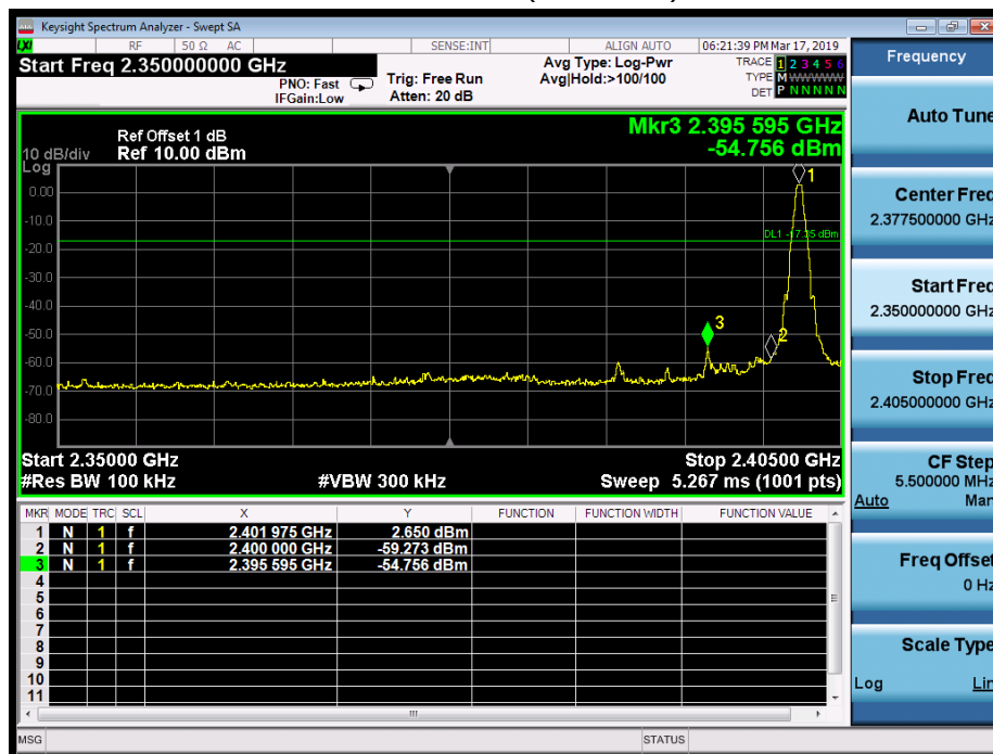
Mode1 CH00(2402MHz)
