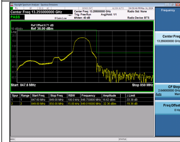
Band5_1.4MHz_16QAM_20643_1RB#5
