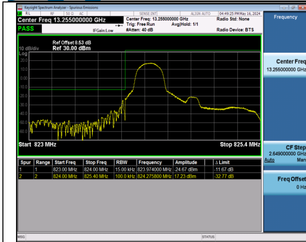
Band5_1.4MHz_16QAM_20407_1RB#0
