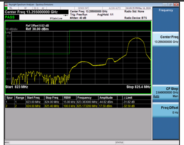
Band5_1.4MHz_QPSK_20407_1RB#5
