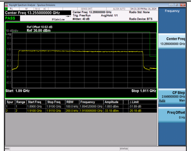
Band2_20MHz_QPSK_19100_100RB#0
