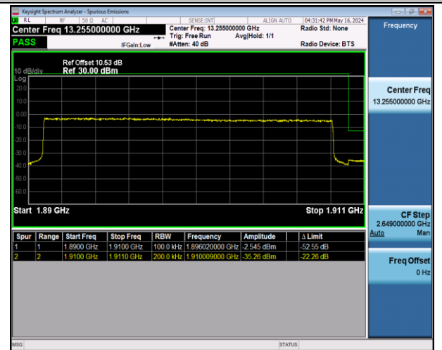
Band2_20MHz_16QAM_19100_100RB#0
