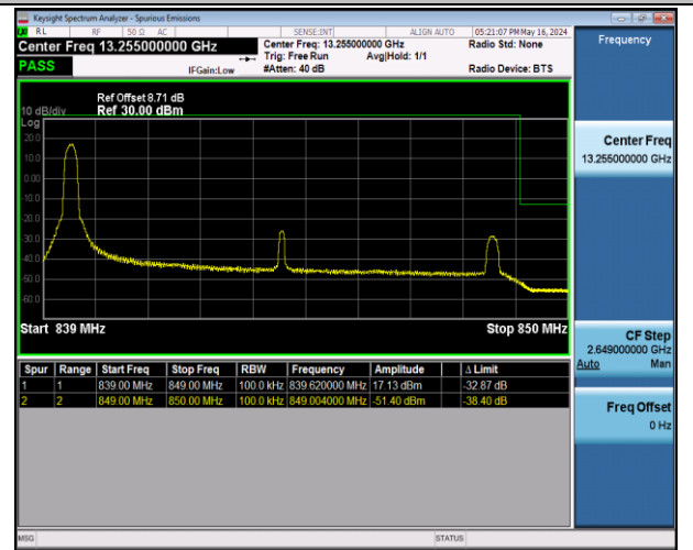
Band5_10MHz_QPSK_20600_1RB#0
