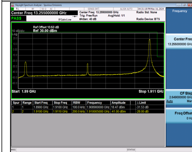
Band2_20MHz_16QAM_19100_1RB#99
