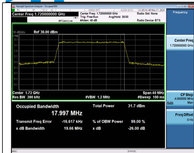
Band66-20MHz-QPSK-132072-100RB#0-PASS
