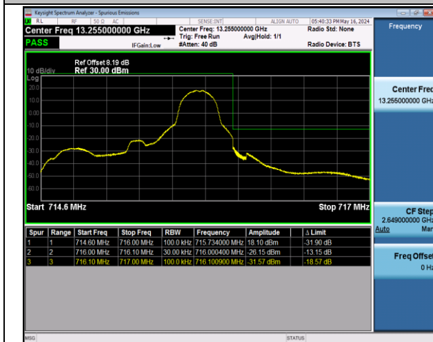
Band12_1.4MHz_QPSK_23173_1RB#5
