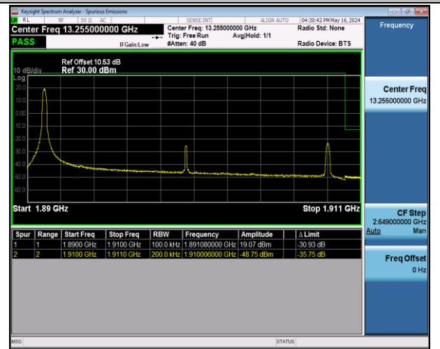
Band2_20MHz_QPSK_19100_1RB#0
