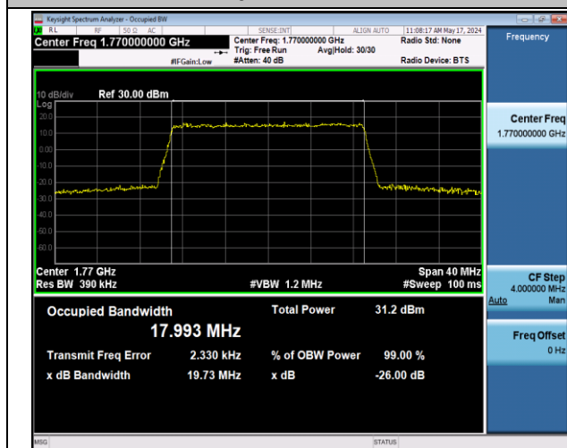
Band66-20MHz-QPSK-132572-100RB#0-PASS
