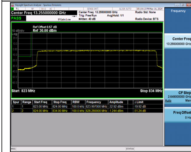
Band5_10MHz_QPSK_20450_50RB#0
