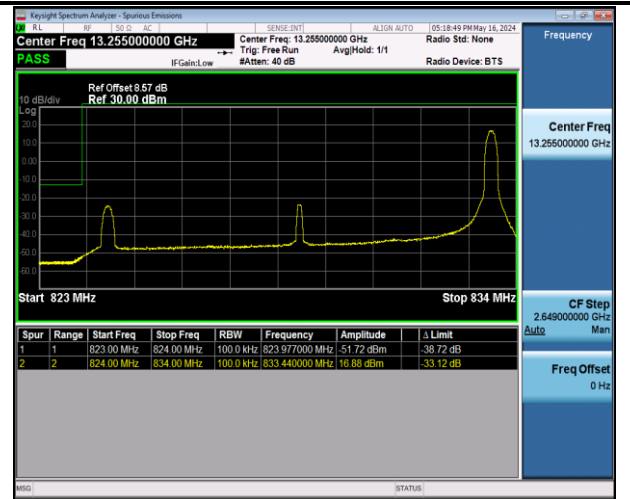
Band5_10MHz_QPSK_20450_1RB#49
