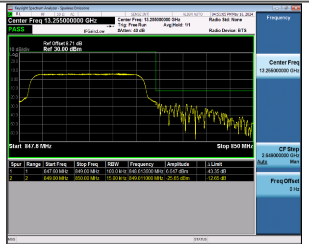
Band5_1.4MHz_16QAM_20643_6RB#0
