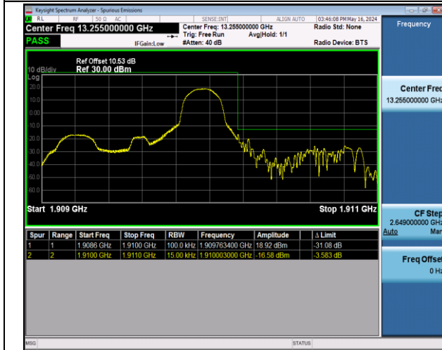
Band2_1.4MHz_16QAM_19193_1RB#5
