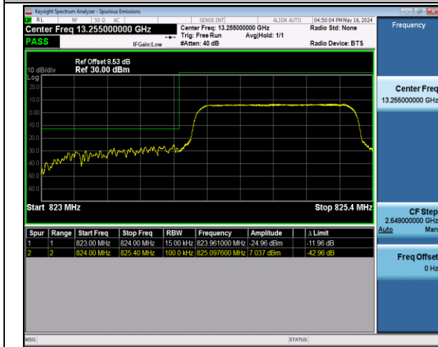
Band5_1.4MHz_16QAM_20407_6RB#0
