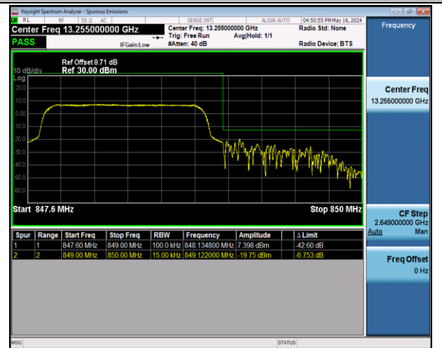
Band5_1.4MHz_QPSK_20643_6RB#0
