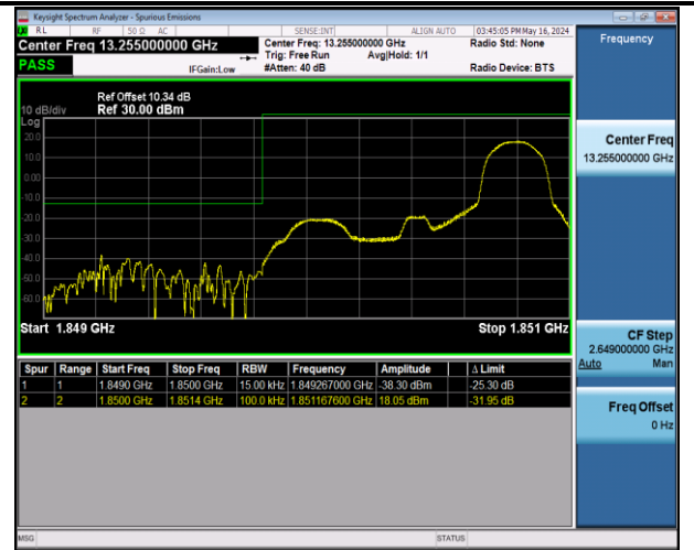
Band2_1.4MHz_16QAM_18607_1RB#5
