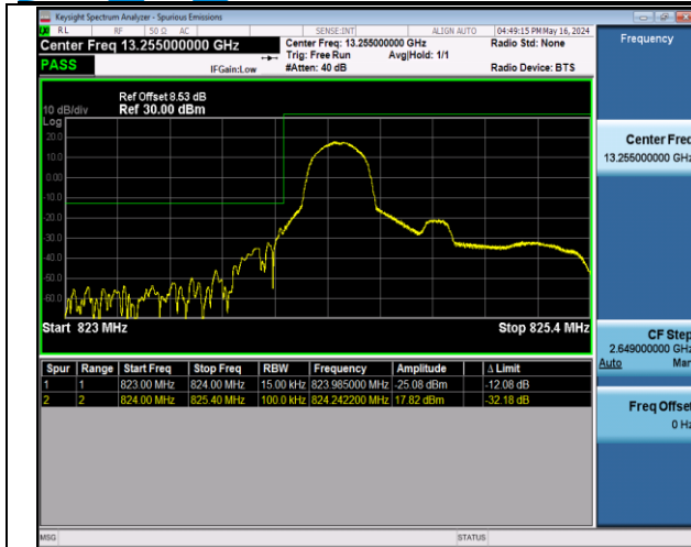
Band5_1.4MHz_QPSK_20407_1RB#0
