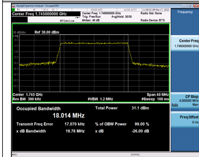
Band66-20MHz-16QAM-132322-100RB#0-PASS
