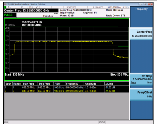
Band5_10MHz_QPSK_20600_50RB#0
