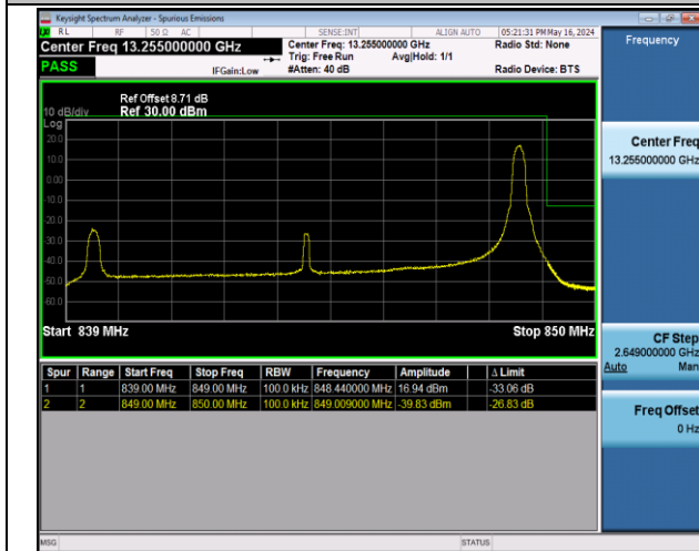
Band5_10MHz_QPSK_20600_1RB#49
