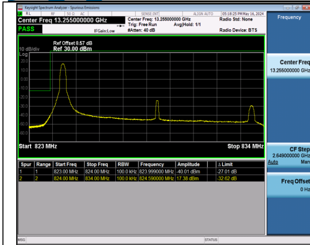
Band5_10MHz_QPSK_20450_1RB#0
