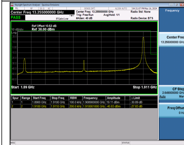
Band2_20MHz_QPSK_19100_1RB#99
