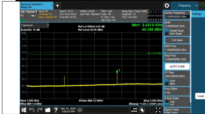
Band13-10MHz-QPSK-23230-1RB#0-1000~3000-PASS
