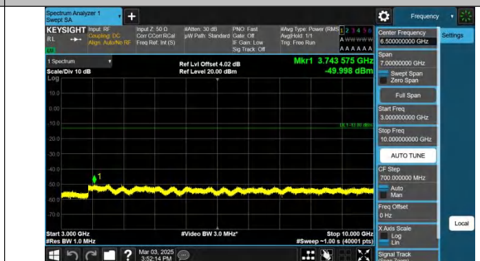
Band13-5MHz-QPSK-23255-1RB#0-3000~10000-PASS
