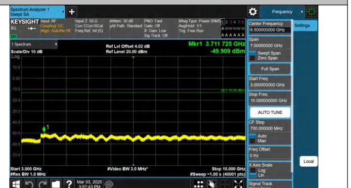
Band13-10MHz-QPSK-23230-1RB#49-3000~10000-PASS
