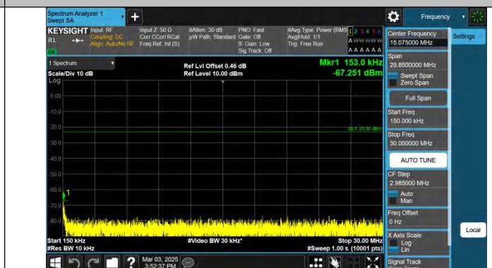
Band13-5MHz-QPSK-23255-1RB#24-0.15~30-PASS
