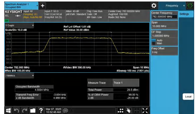
Band13-5MHz-16QAM-23230-25RB#0-PASS
