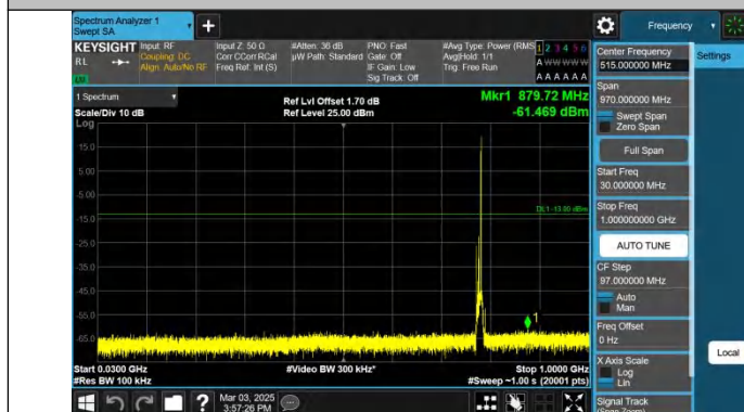
Band13-10MHz-QPSK-23230-1RB#49-30~1000-PASS
