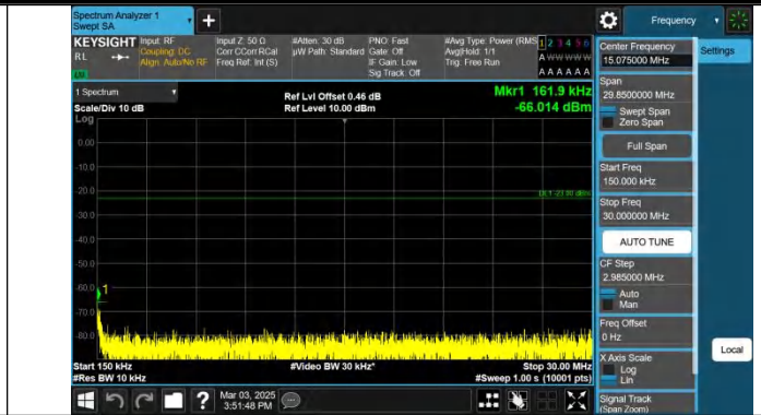
Band13-5MHz-QPSK-23255-1RB#0-0.15~30-PASS
