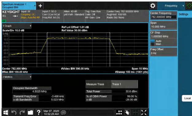
Band13-5MHz-QPSK-23230-25RB#0-PASS
