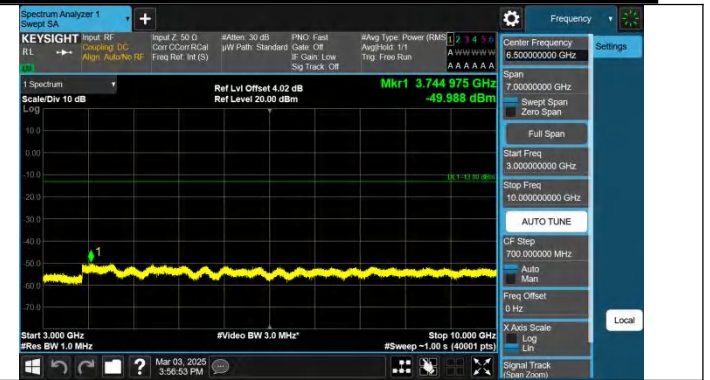
Band13-10MHz-QPSK-23230-1RB#0-3000~10000-PASS
