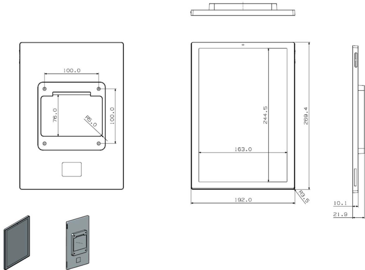
Figure 12. 11.6" Mechanical Dimension
