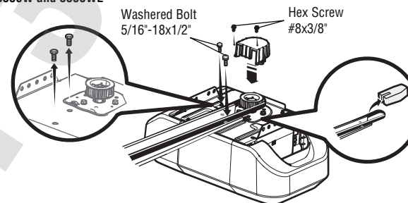
Washer Bolt 5/16"-18x1/2" (Mounted in the garage door opener) Models 8550W and 8550WL (2) Model 8557W (1)
