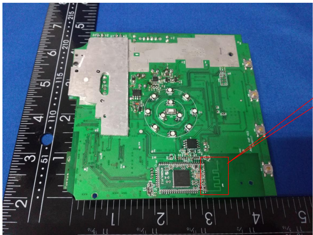
BT Antenna
