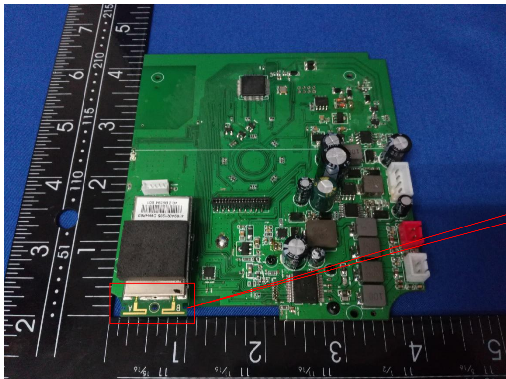
5G Antenna
