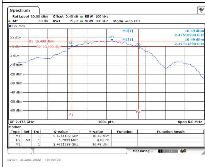
O-QPSK / 2475 MHz
