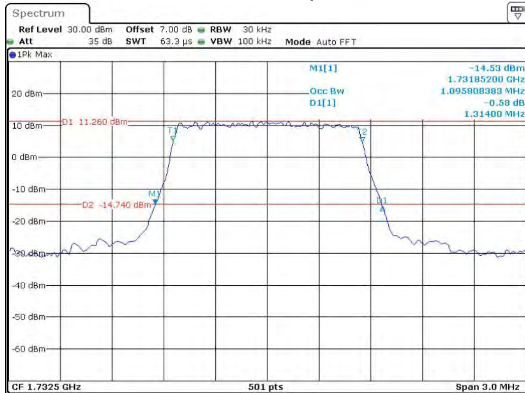
Band 4_1.4 MHz_Middle_QPSK_RB6#0
