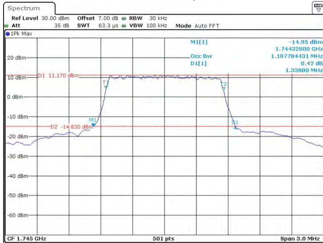
Band 66_1.4 MHz_Middle_QPSK_RB6#0
