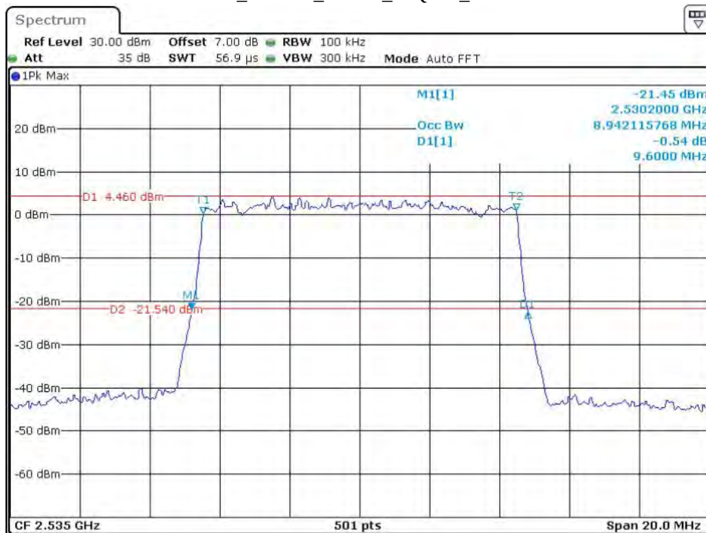
Band 7_10 MHz_Middle_16QAM_RB50#0
