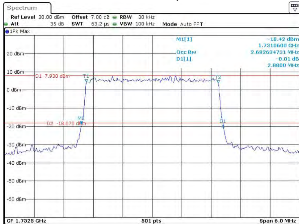
Band 4_3 MHz_Middle_16QAM_RB15#0
