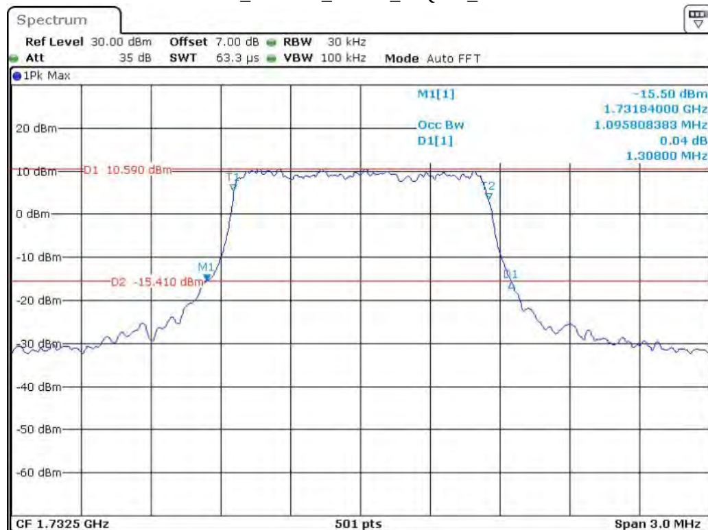
Band 4_1.4 MHz_Middle_16QAM_RB6#0
