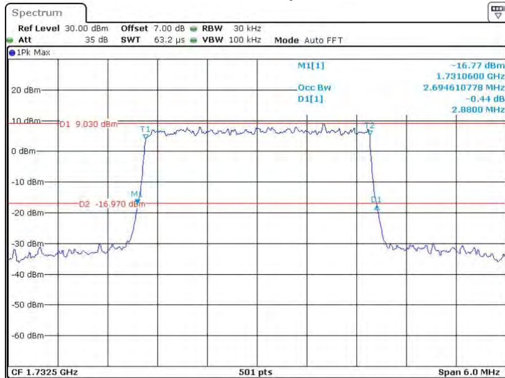
Band 4_3 MHz_Middle_QPSK_RB15#0
