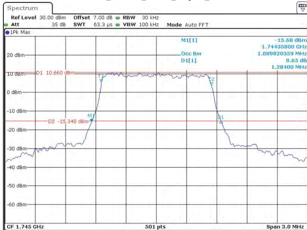
Band 66_1.4 MHz_Middle_16QAM_RB6#0
