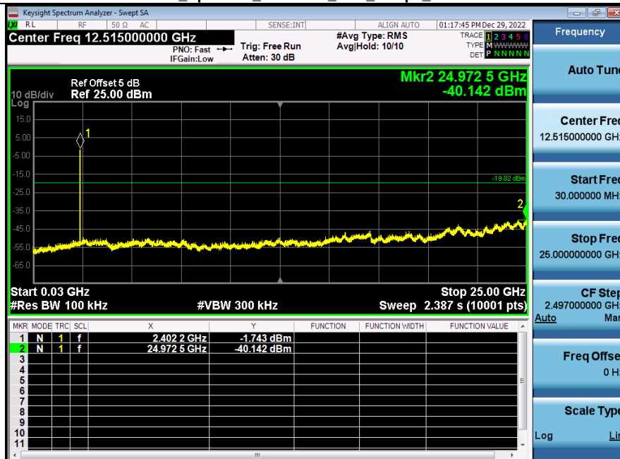
2_Spurious_Emission_BLE_1Mbps_2402
