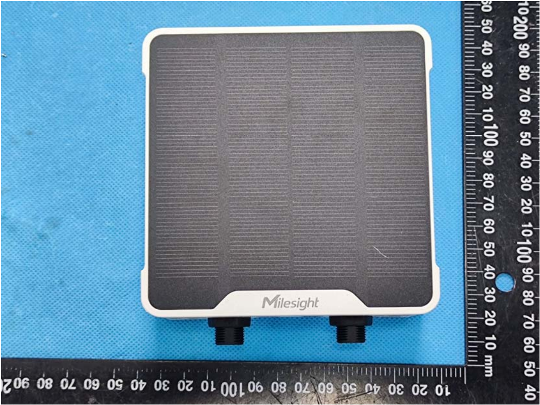
Model: UC501-915M (Series models: UC501-9M, NC501-915M, NC501-9M are identical with this model)
