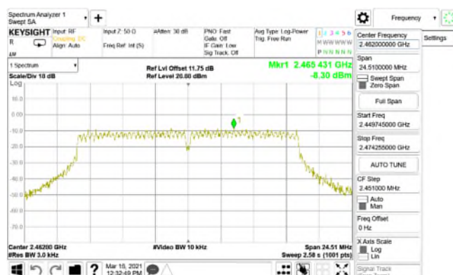
Power Density_802.11g_20MHz_Chain1_2462MHz
