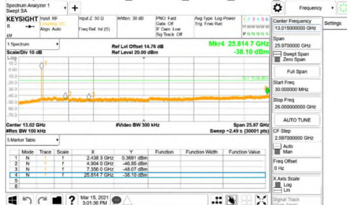
Spurious Emission_802.11ax_40MHz_Chain0_2452MHz
