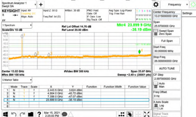
Spurious Emission_802.11n_40MHz_Chain0_2452MHz
