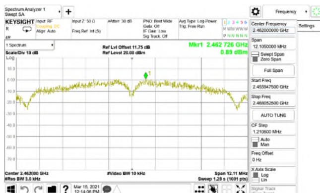
Power Density_802.11b_20MHz_Chain0_2462MHz
