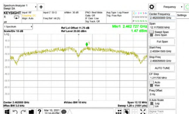
Power Density_802.11b_20MHz_Chain1_2462MHz
