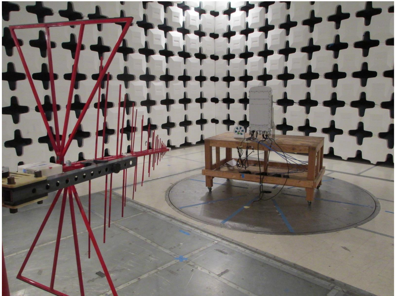
RE – 30-1000MHz at 3m
