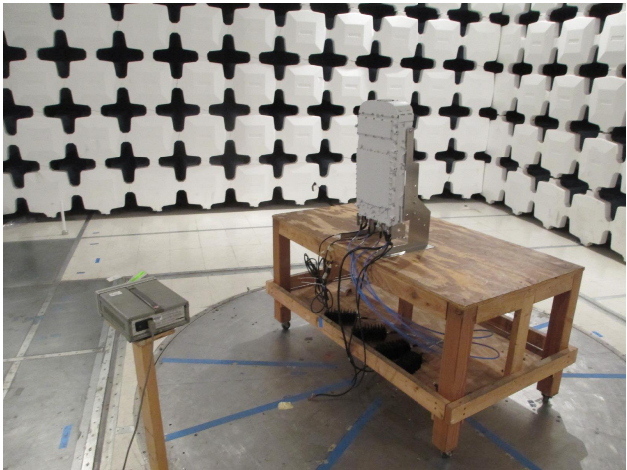
RE – 18-22GHz
