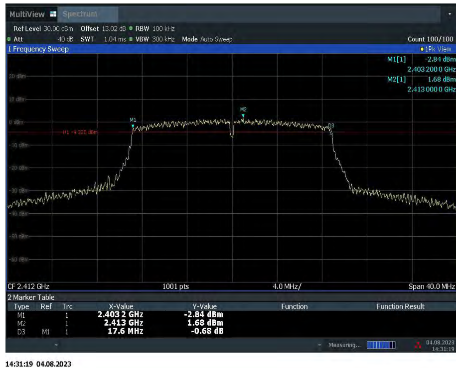
Fig.A.4.7 Occupied 6dB Bandwidth (802.11n-HT20, Ch 1)
