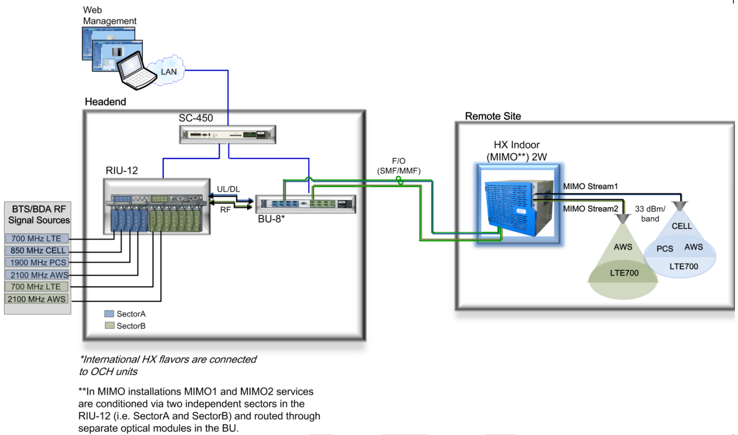
Example of Indoor MIMO Architecture with HX Quad-Band
