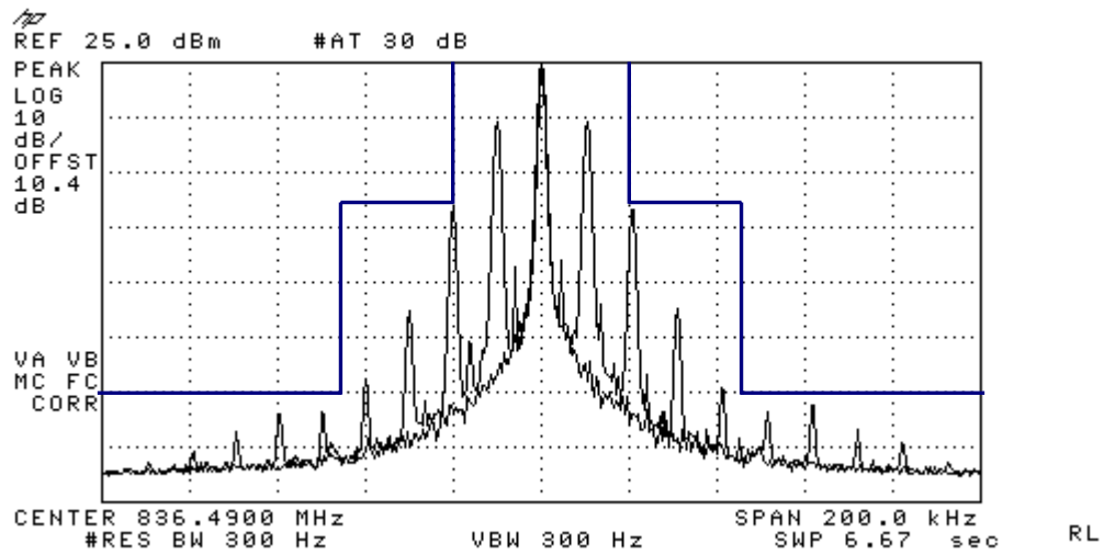
Figure 7-4 AMPS ST
