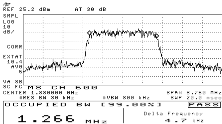
Figure 7-9 CDMA 1900 @ CH 600
