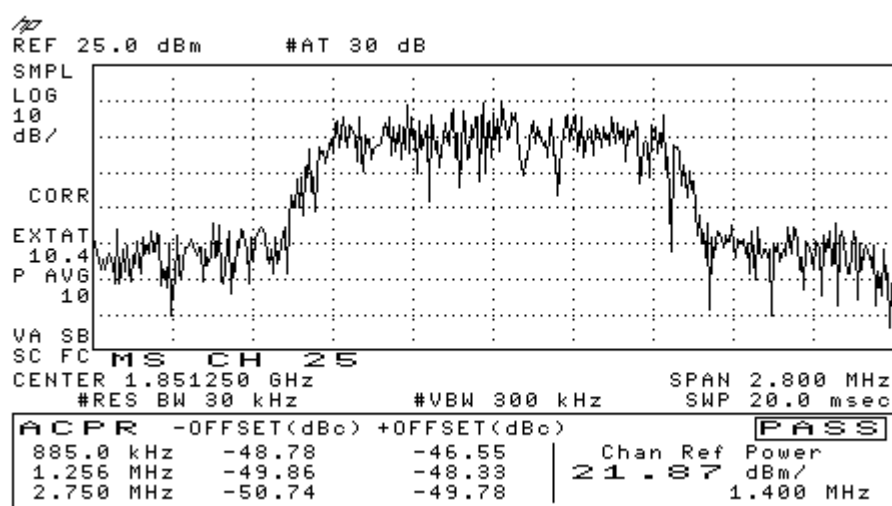
Figure 7-10 CDMA 1900 Lower Band Edge
