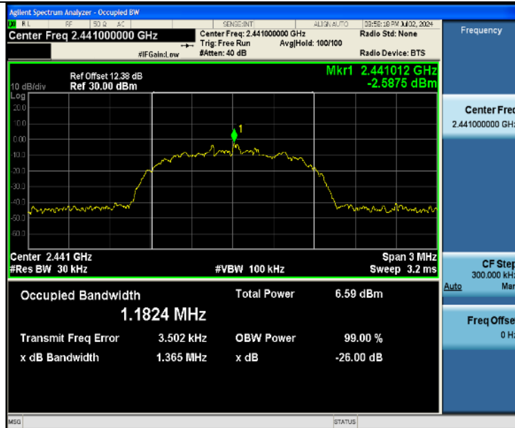
3DH5-Ant1-2441
