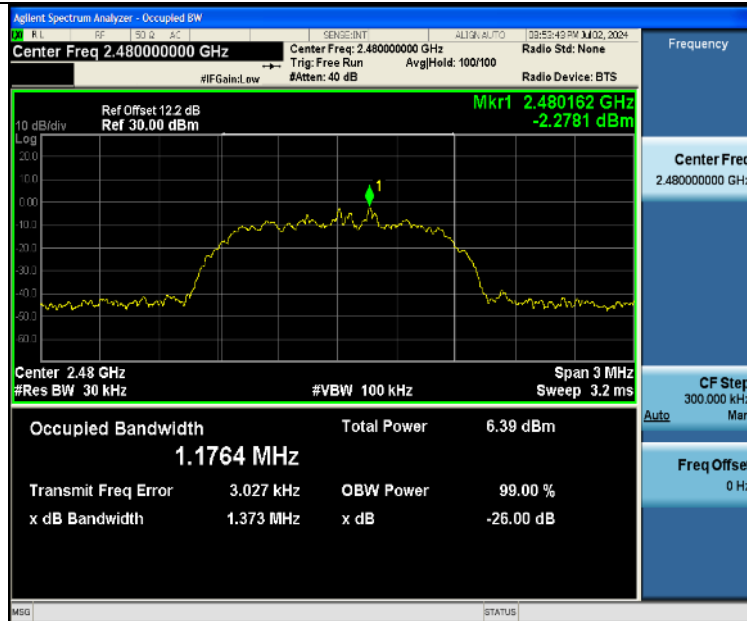
2DH5-Ant1-2480
