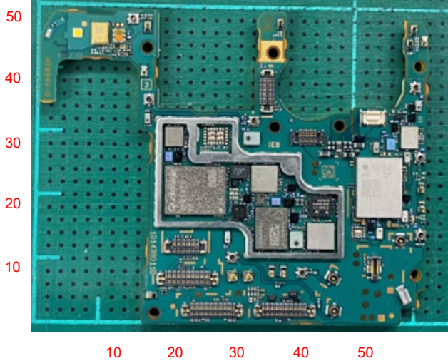
Internal Main-PWB Rear without Shield case (Rear-side)
