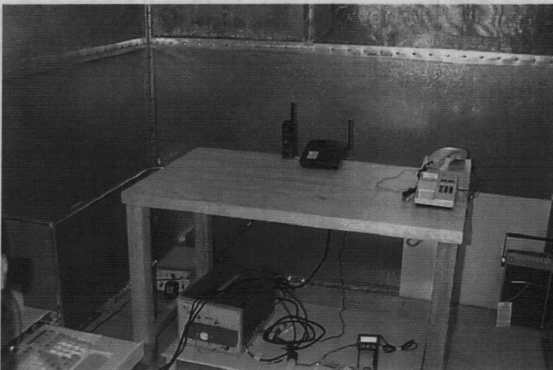
Figure D.1.1 Conducted Emissions Test Configuration Photos
