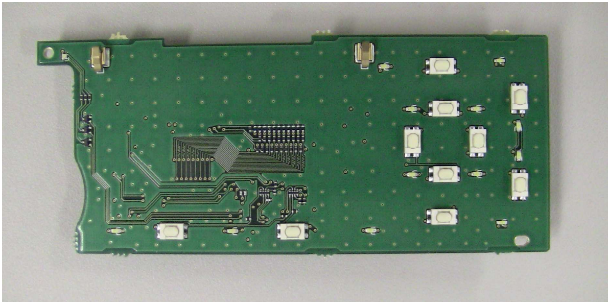
IC-F7540 FRONT-A UNIT A SIDE
