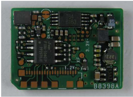
IC-F7540 AES/DES UNIT (UT-134) SIDE A
