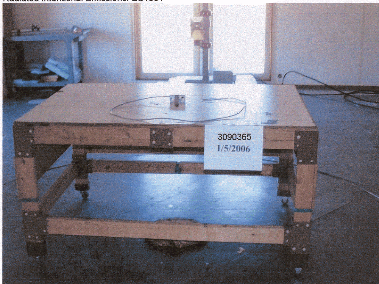
Test-setup photo(s): Radiated Intentional Emissions: ES1501
