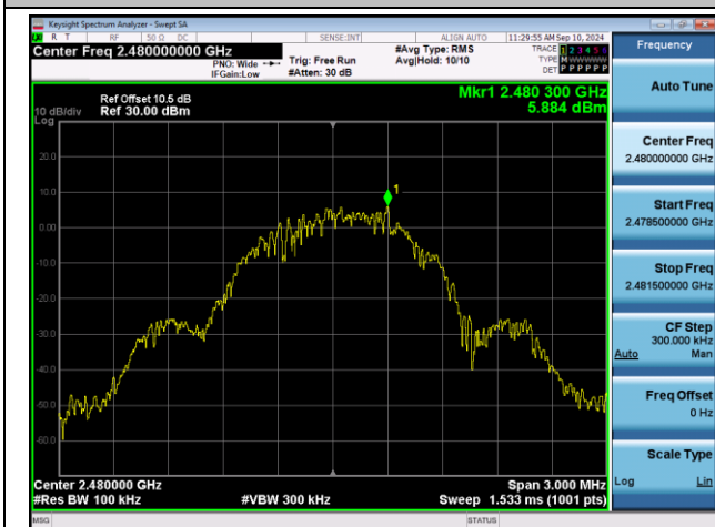
BLE_1M-Ant1-2480-0~Reference-PASS
