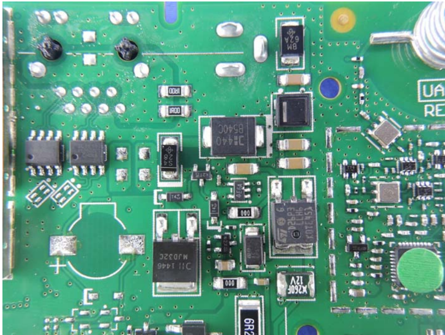
(25) EUT Photo
