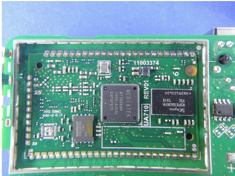
(22) EUT Photo
