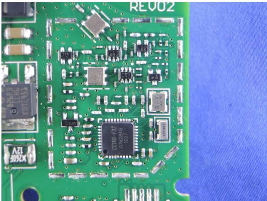
(26) EUT Photo
