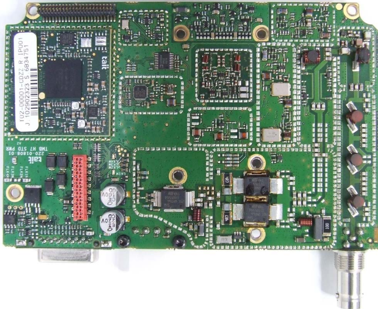
Photograph 02: Radio - Main PCB top without shields
