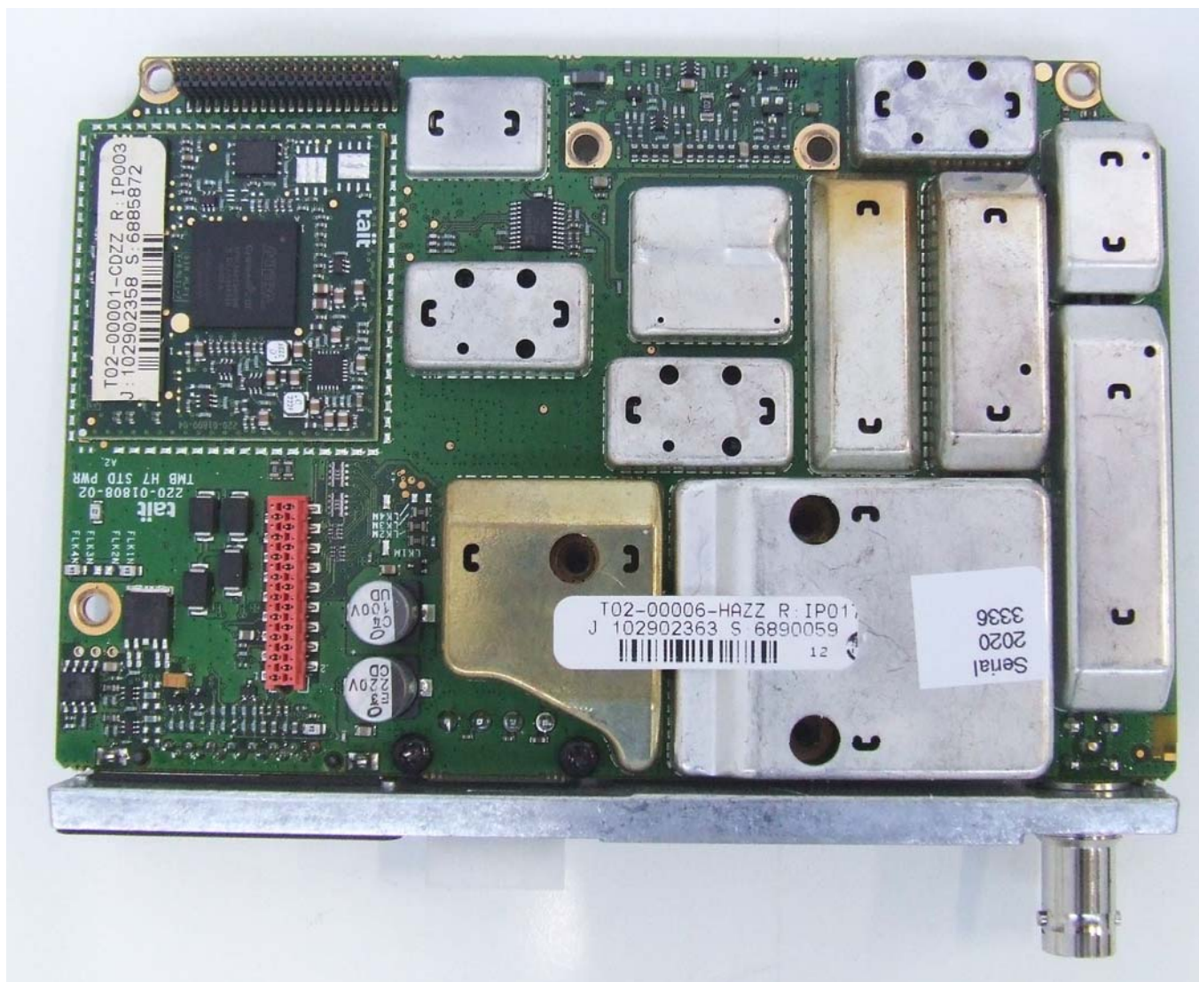
Photograph 01: Radio - Main PCB top with shields
