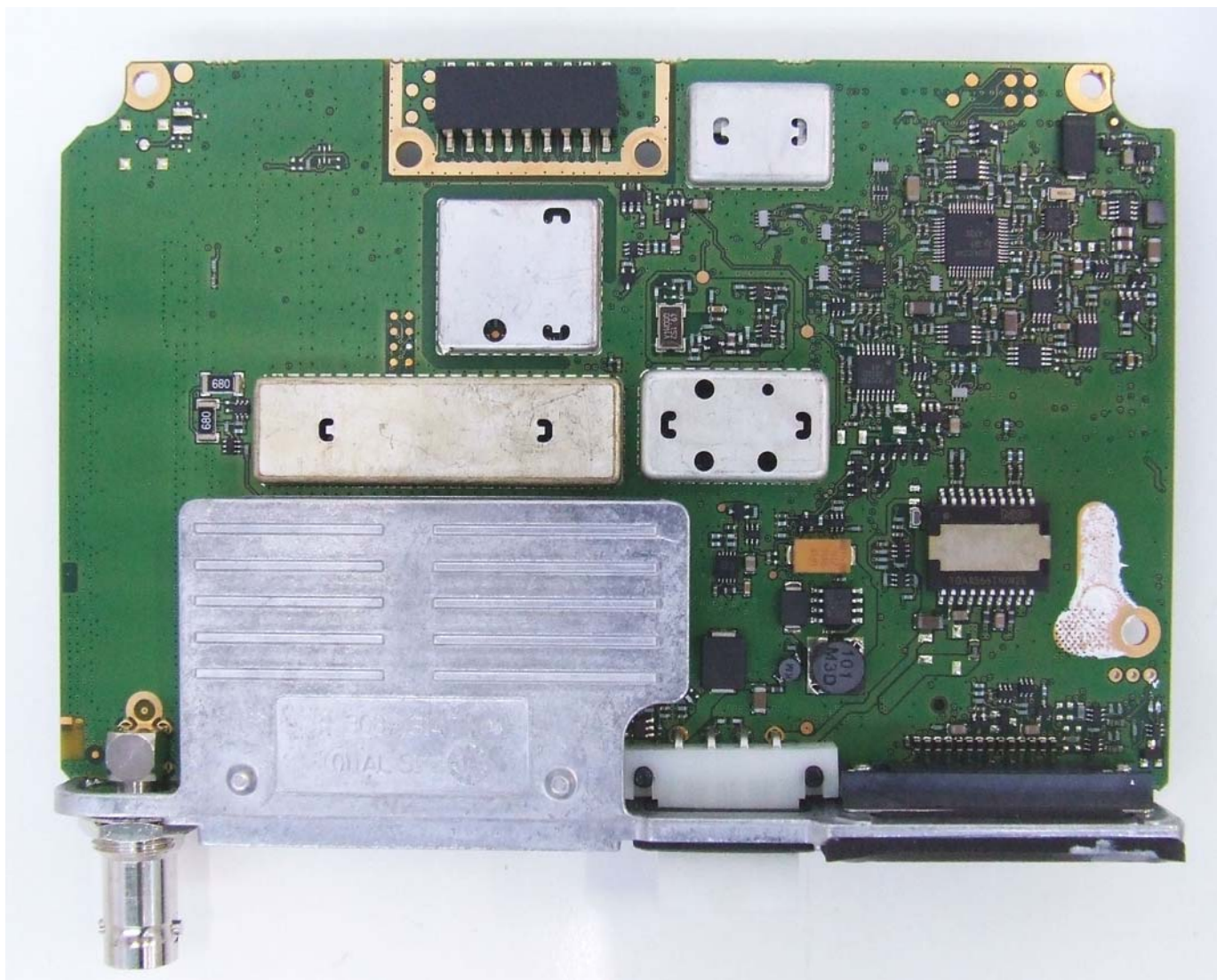
Photograph 03: Radio - Main PCB bottom with shields
