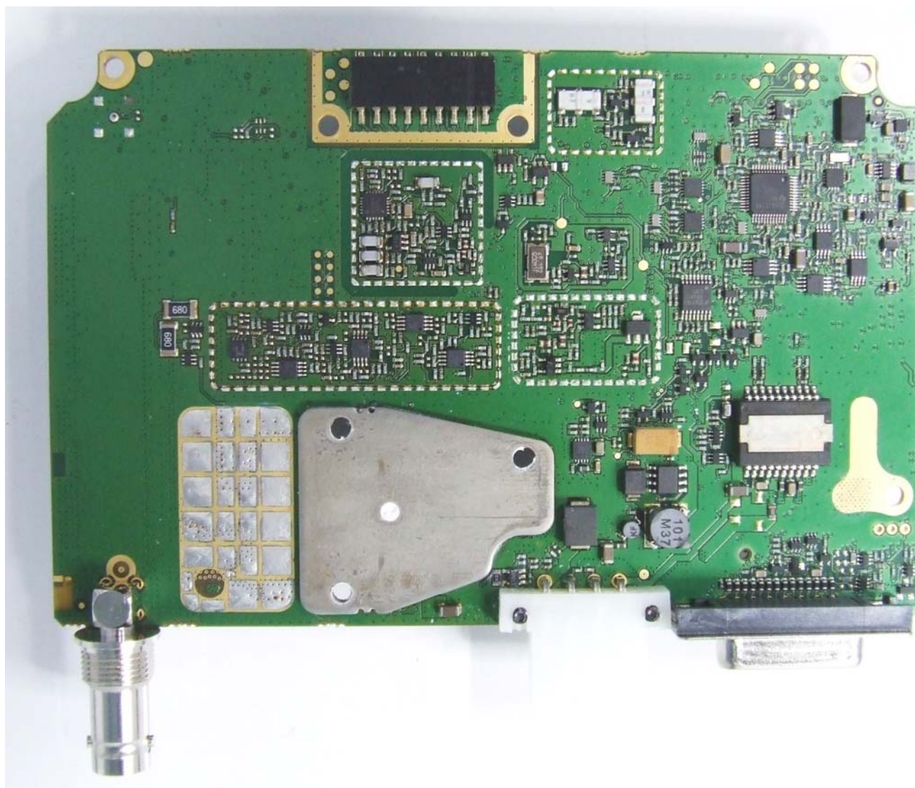
Photograph 04: Radio - Main PCB bottom without shields
