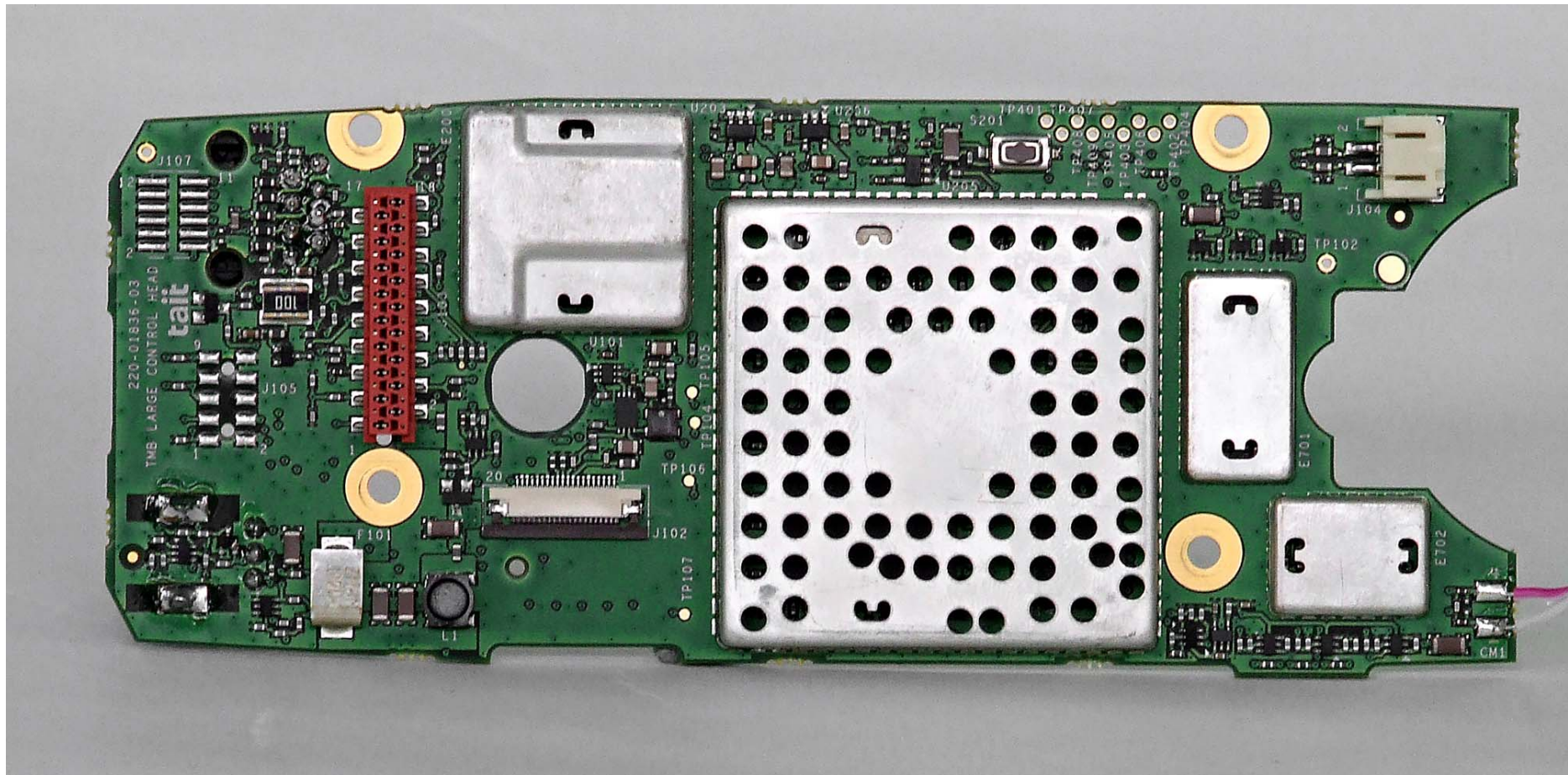
Photograph 07: Control Head - main PCB top with shields
