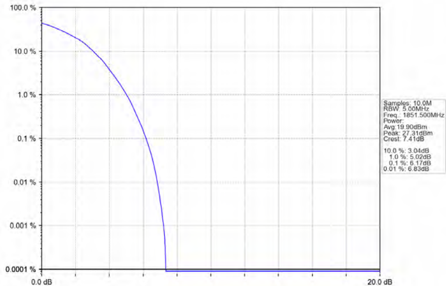
Band2_3MHz_64QAM_LCH_1851.5MHz_RB_15_0_NTNV
