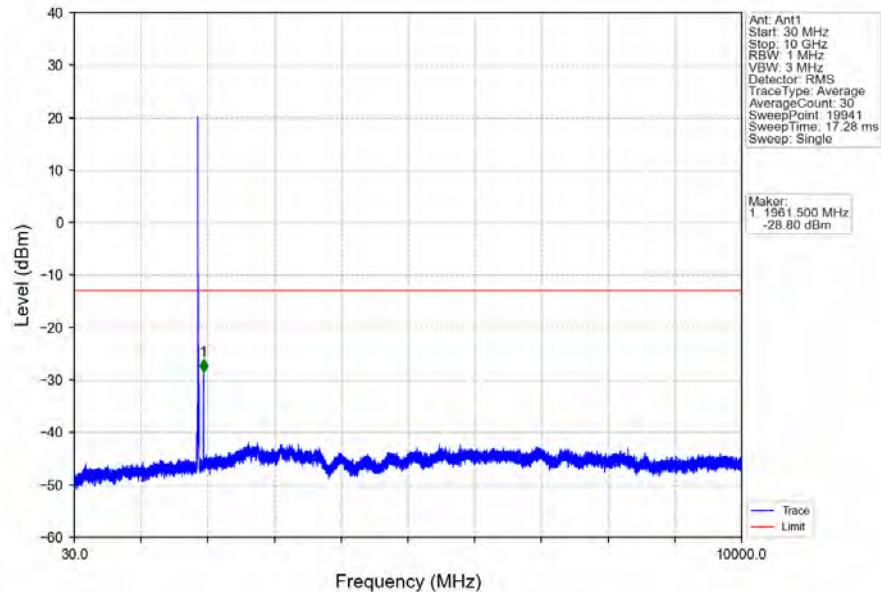
Band2_10MHz_64QAM_MCH_1880MHz_RB_1_0_NTNV
