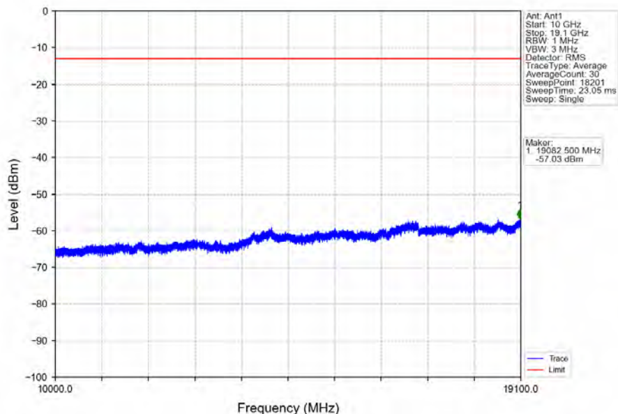
Band2_5MHz_64QAM_MCH_1880MHz_RB_1_0_NTNV
