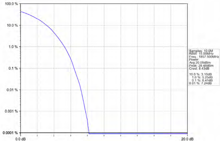
Band2_15MHz_64QAM_LCH_1857.5MHz_RB_75_0_NTNV
