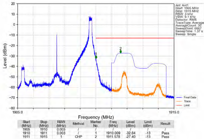
Band2_5MHz_16QAM_HCH_1907.5MHz_RB_1_24_NTNV
