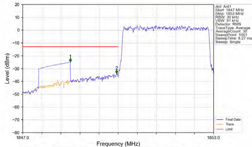
Band2_3MHz_16QAM_LCH_1851.5MHz_RB_15_0_NTNV
