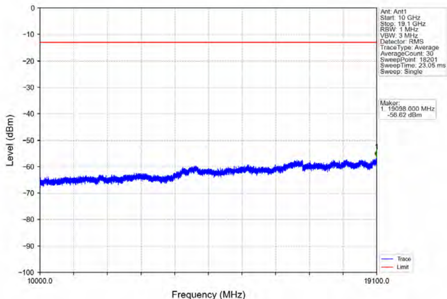
Band2_1.4MHz_16QAM_MCH_1880MHz_RB_1_0_NTNV
