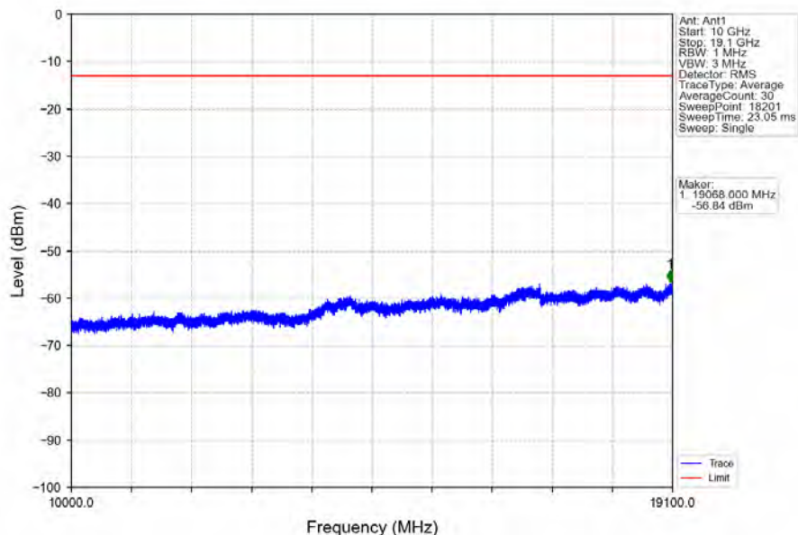
Band2_1.4MHz_64QAM_HCH_1909.3MHz_RB_1_0_NTNV
