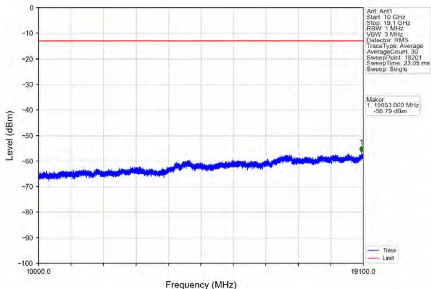
Band2_3MHz_64QAM_HCH_1908.5MHz_RB_1_0_NTNV
