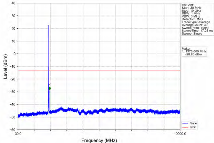
Band2_15MHz_16QAM_HCH_1902.5MHz_RB_1_0_NTNV
