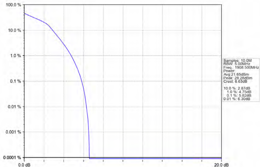
Band2_3MHz_16QAM_HCH_1908.5MHz_RB_15_0_NTNV
