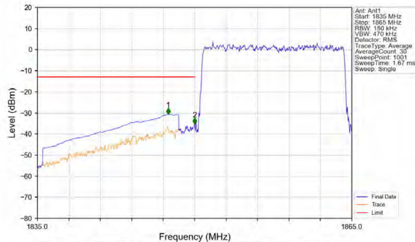
Band2_15MHz_64QAM_LCH_1857.5MHz_RB_75_0_NTNV
