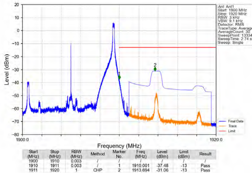
Band2_10MHz_64QAM_HCH_1905MHz_RB_1_49_NTNV
