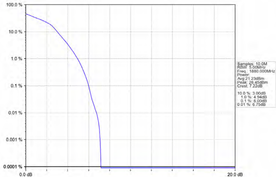
Band2_1.4MHz_16QAM_MCH_1880MHz_RB_6_0_NTNV
