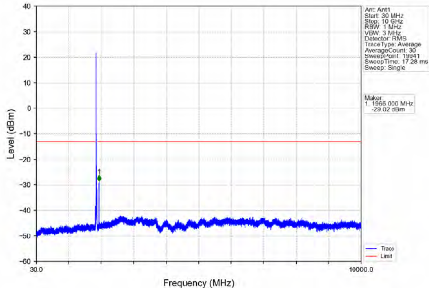
Band2_15MHz_64QAM_MCH_1880MHz_RB_1_0_NTNV
