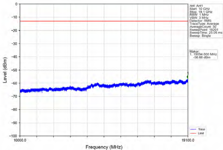
Band2_15MHz_64QAM_HCH_1902.5MHz_RB_1_0_NTNV
