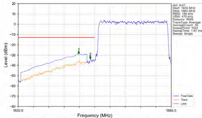
Band2_15MHz_16QAM_LCH_1857.5MHz_RB_75_0_NTNV
