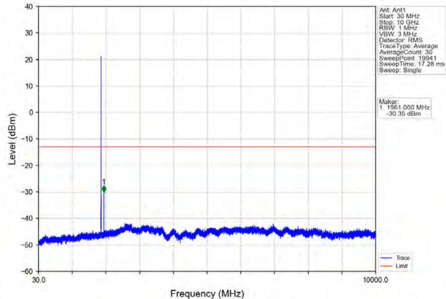
Band2_3MHz_64QAM_MCH_1880MHz_RB_1_0_NTNV
