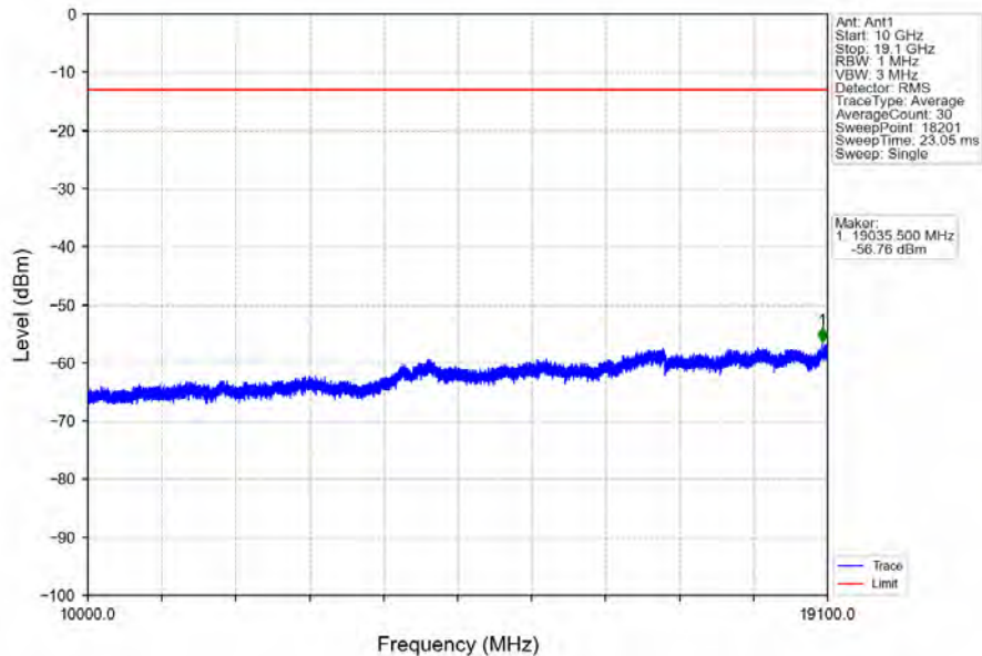
Band2_15MHz_16QAM_LCH_1857.5MHz_RB_75_0_NTNV
