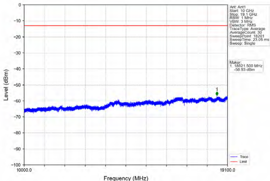
Band2_3MHz_64QAM_MCH_1880MHz_RB_1_0_NTNV
