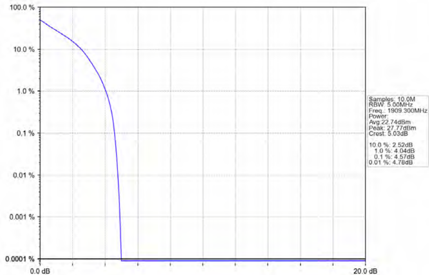
Band2_1.4MHz_QPSK_HCH_1909.3MHz_RB_6_0_NTNV
