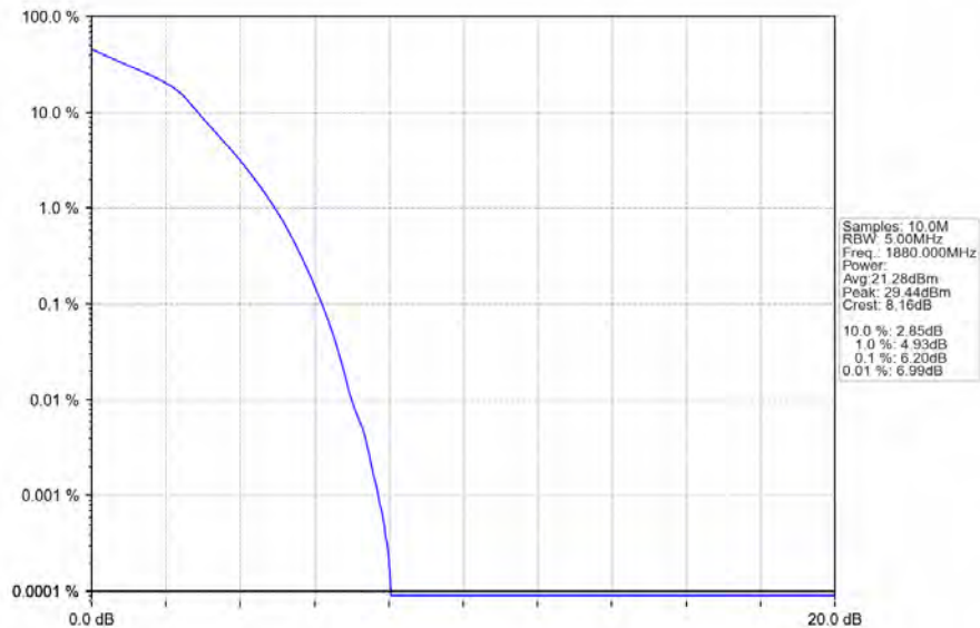
Band2_5MHz_16QAM_MCH_1880MHz_RB_25_0_NTNV
