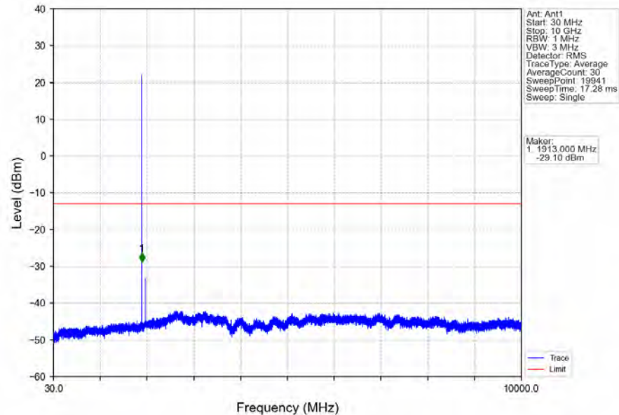
Band2_1.4MHz_16QAM_HCH_1909.3MHz_RB_1_0_NTNV
