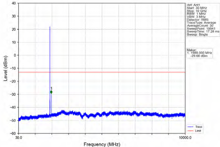
Band2_5MHz_64QAM_HCH_1907.5MHz_RB_1_0_NTNV
