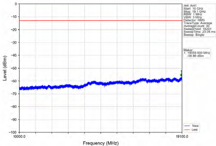
Band2_10MHz_64QAM_HCH_1905MHz_RB_1_0_NTNV
