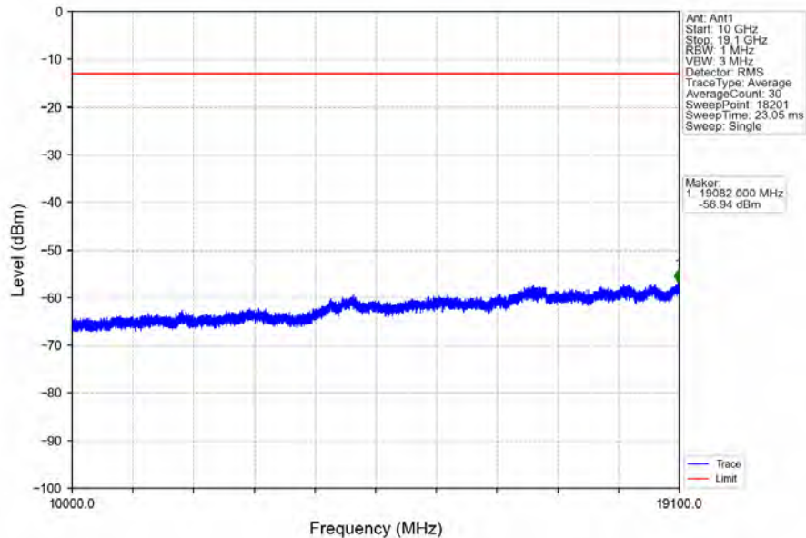
Band2_1.4MHz_16QAM_LCH_1850.7MHz_RB_6_0_NTNV
