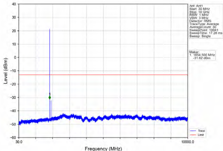
Band2_1.4MHz_16QAM_LCH_1850.7MHz_RB_1_0_NTNV
