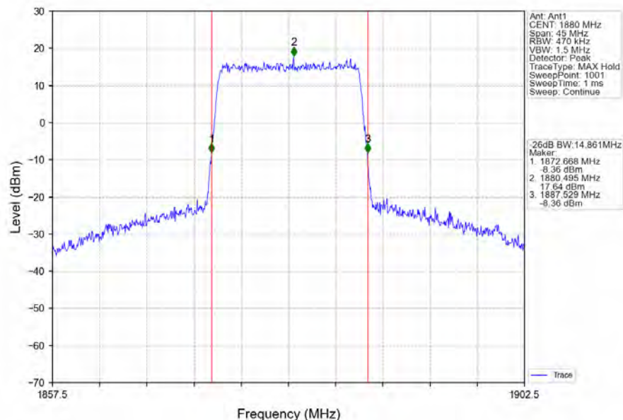
Band2_15MHz_64QAM_MCH_1880MHz_RB_75_0_NTNV
