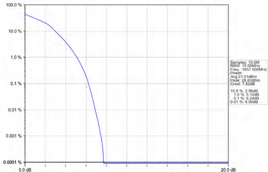
Band2_15MHz_16QAM_LCH_1857.5MHz_RB_75_0_NTNV
