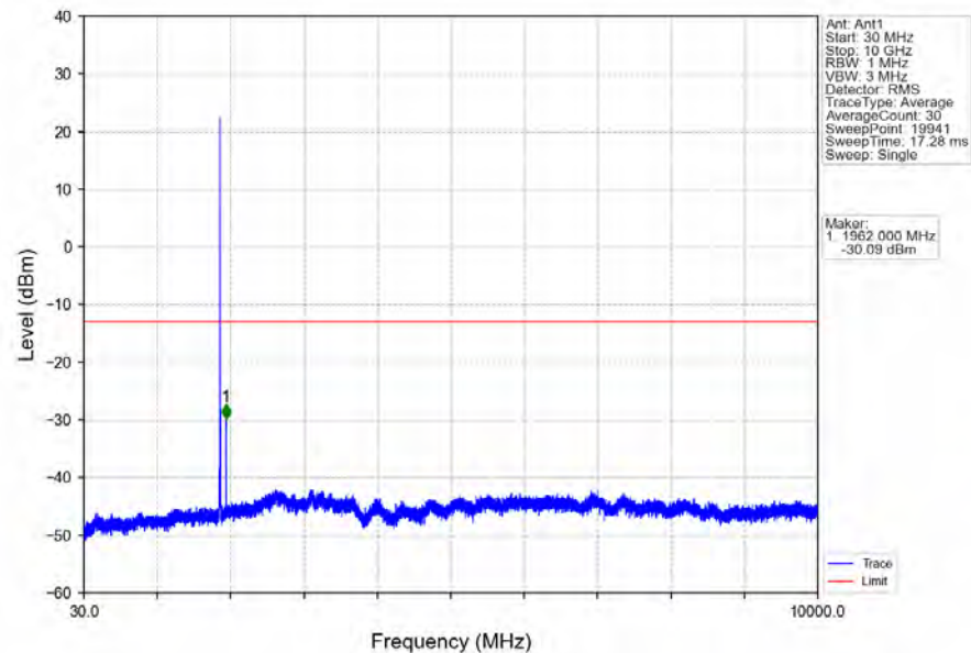
Band2_5MHz_16QAM_MCH_1880MHz_RB_1_0_NTNV
