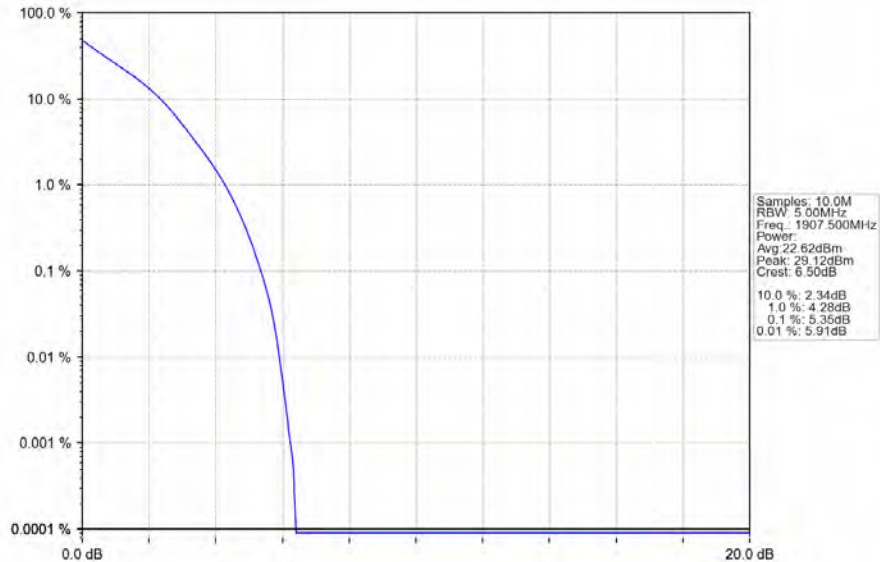
Band2_5MHz_QPSK_HCH_1907.5MHz_RB_25_0_NTNV
