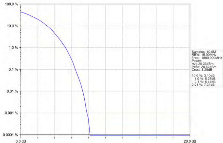
Band2_15MHz_64QAM_MCH_1880MHz_RB_75_0_NTNV
