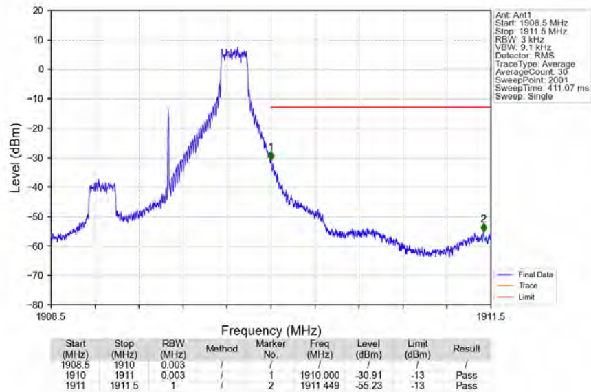
Band2_1.4MHz_16QAM_HCH_1909.3MHz_RB_1_5_NTNV
