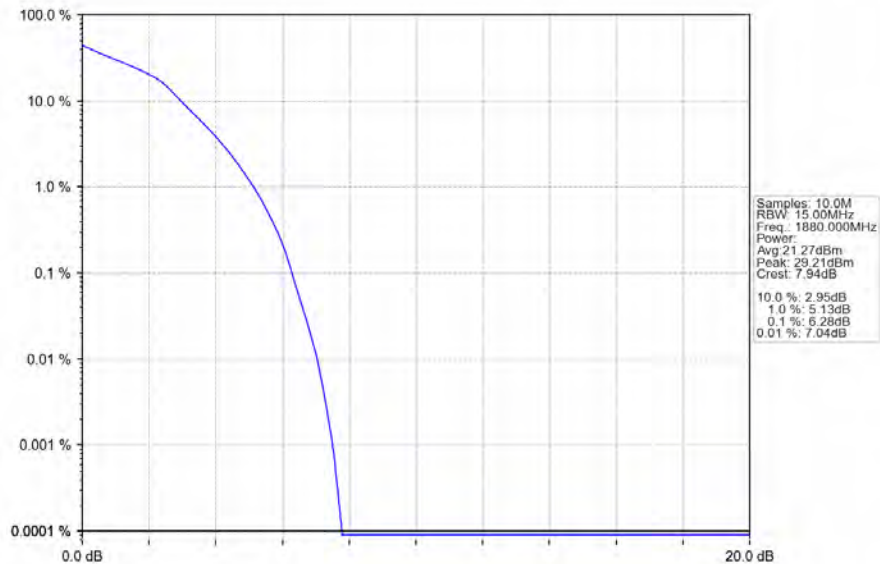
Band2_15MHz_16QAM_MCH_1880MHz_RB_75_0_NTNV
