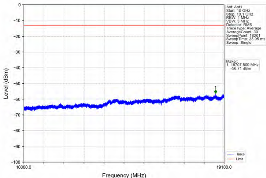
Band2_10MHz_64QAM_MCH_1880MHz_RB_1_0_NTNV
