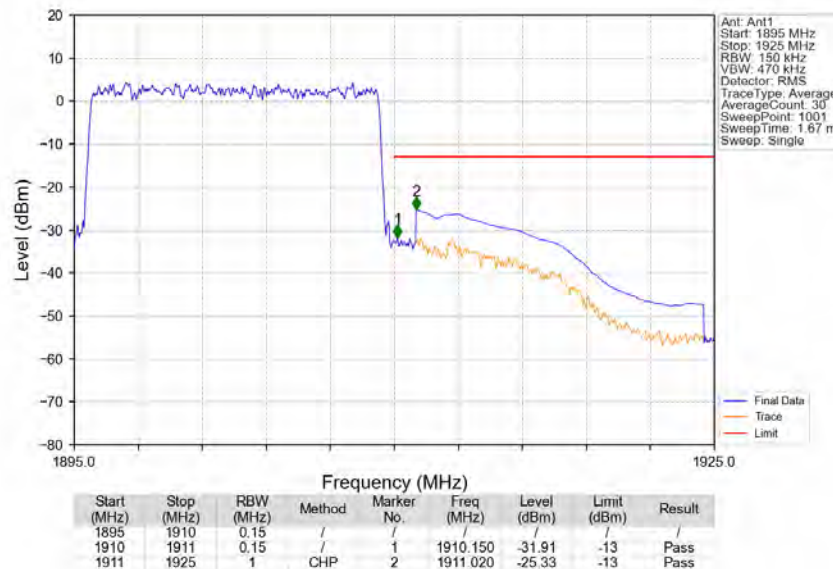
Band2_15MHz_16QAM_HCH_1902.5MHz_RB_75_0_NTNV
