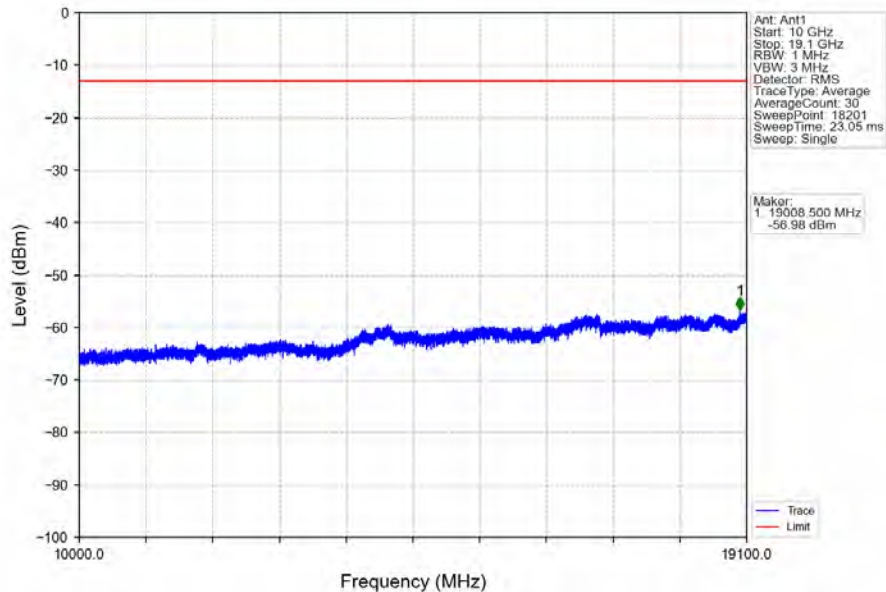
Band2_15MHz_QPSK_LCH_1857.5MHz_RB_75_0_NTNV
