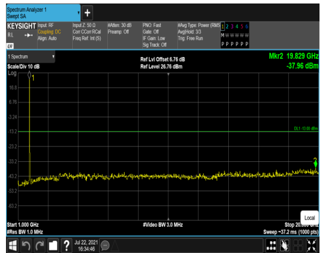
Band4-20MHz-16QAM-20300:1000~20000MHz
