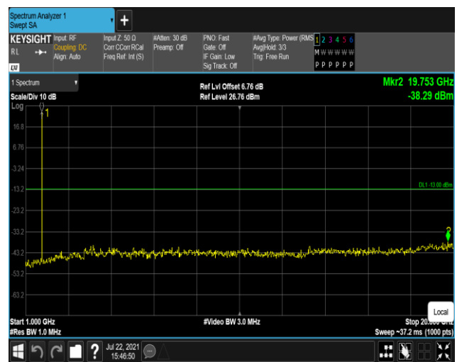
Band4-1.4MHz-16QAM-20393:1000~20000MHz
