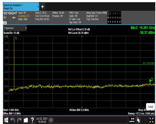
Band4-1.4MHz-16QAM-20175:1000~20000MHz
