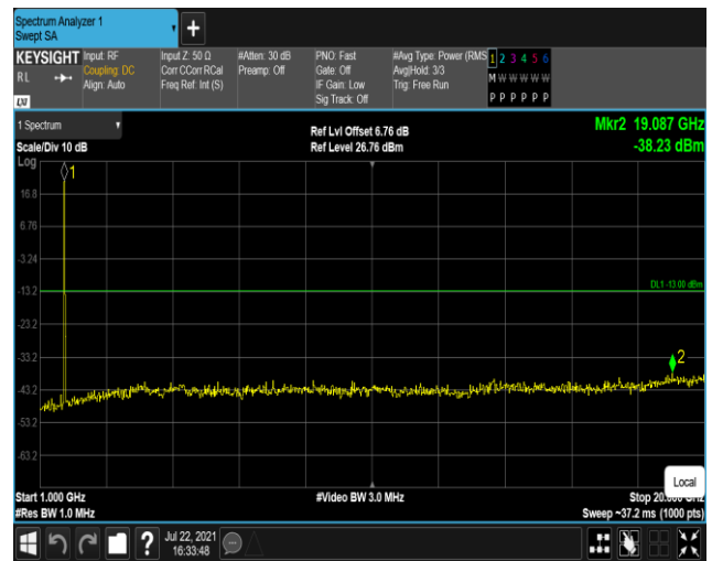
Band4-20MHz-16QAM-20175:1000~20000MHz
