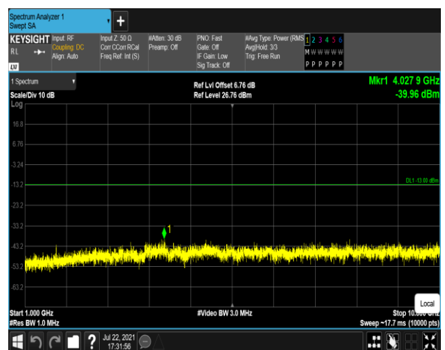
Band5-10MHz-QPSK-20600:1000~10000MHz
