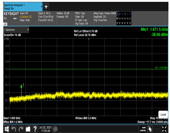
Band5-1.4MHz-16QAM-20643:1000~10000MHz
