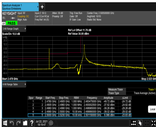
Band7-20MHz-16QAM-20850-100RB#0
