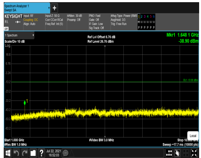
Band5-1.4MHz-16QAM-20525:1000~10000MHz
