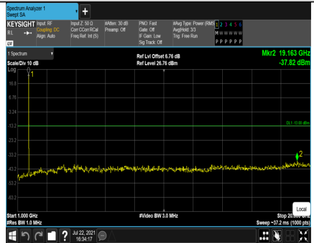
Band4-20MHz-QPSK-20300:1000~20000MHz
