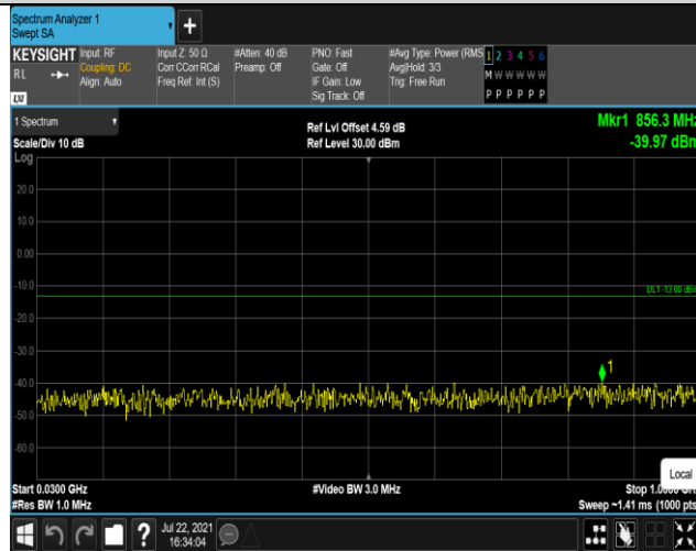
Band4-20MHz-QPSK-20300:30~1000MHz
