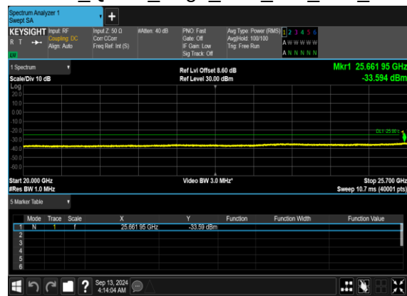
N7(40M)_DFT-s- OFDM_QPSK_Edge_1RB_Left_Low_CH
