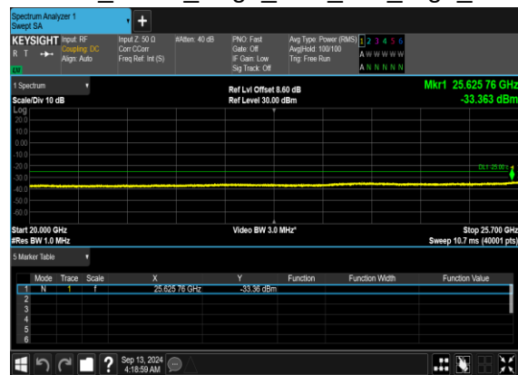
N7(40M)_DFT-s- OFDM_BPSK_Edge_1RB_Left_High_CH
