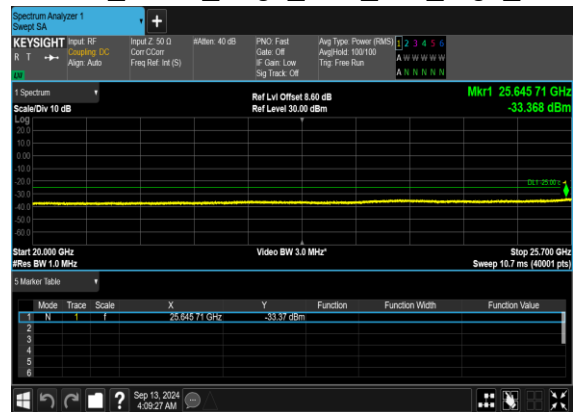
N7(20M)_DFT-s- OFDM_BPSK_Edge_1RB_Left_High_CH
