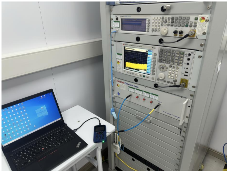
DFS
