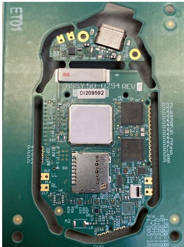
External modem photos Front and back
