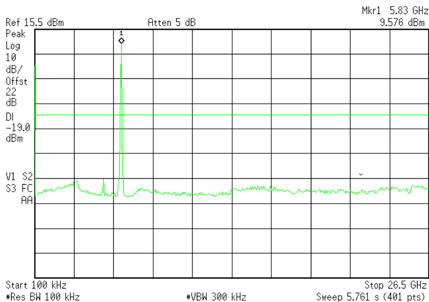
Plot # 31. PRBS 54 Mbit/s. Conducted emission in freq. range 100 kHz - 26.5 GHz/Freq. - HIGH
