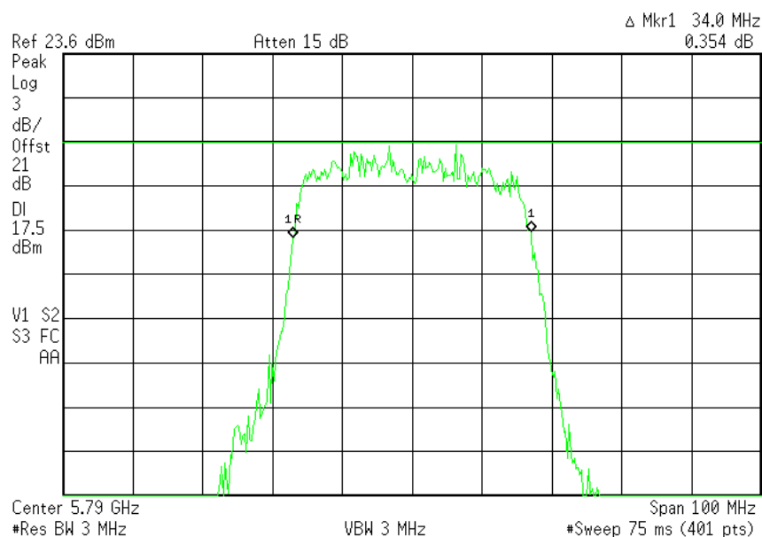
Plot # 18. Freq. - MID
