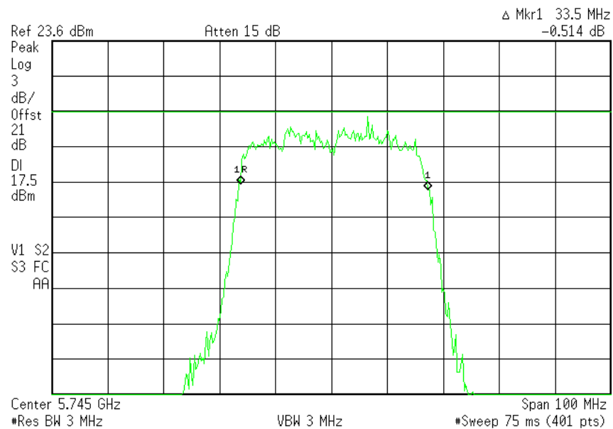
Plot # 17. Freq. – LOW
