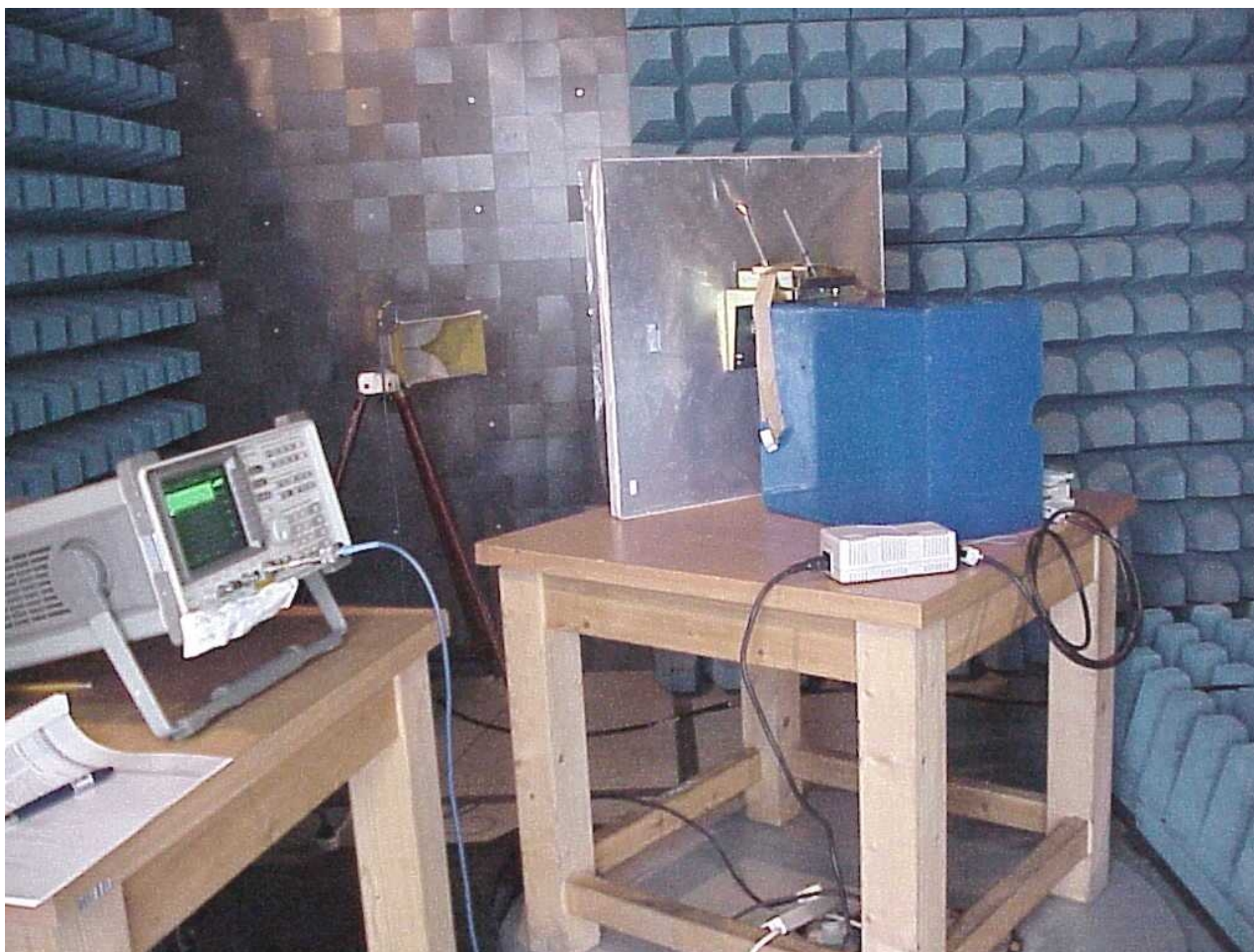
Photo # 1. BreezeNET B unit with Antenna UNI-28-4 P/N 858109. Test setup
