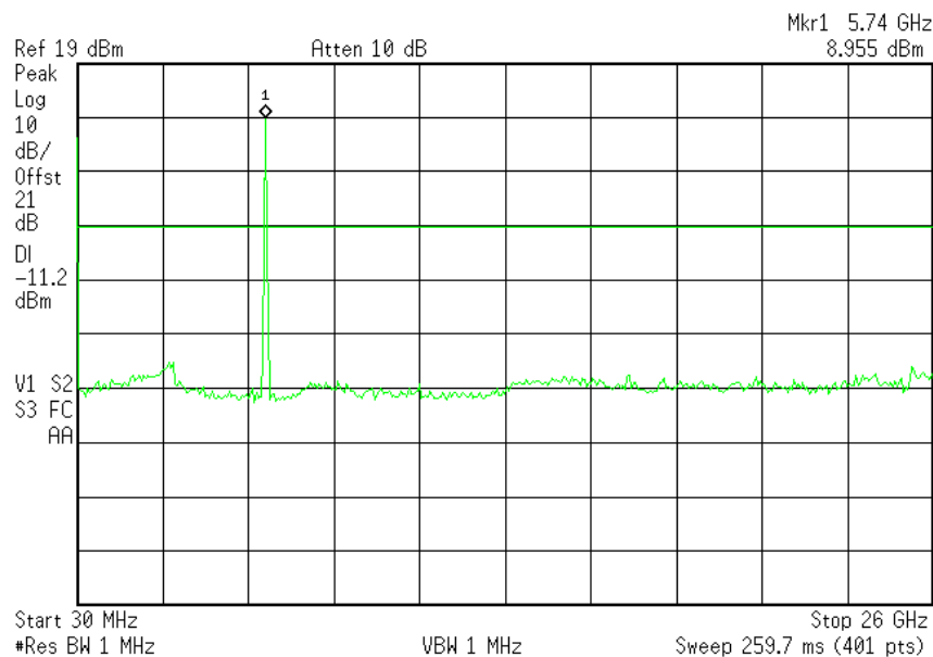
Plot # 26. PRBS 6 Mbit/s.
