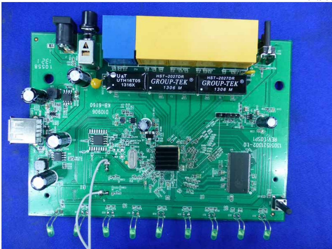
Figure 34 Fontside of the PCB
