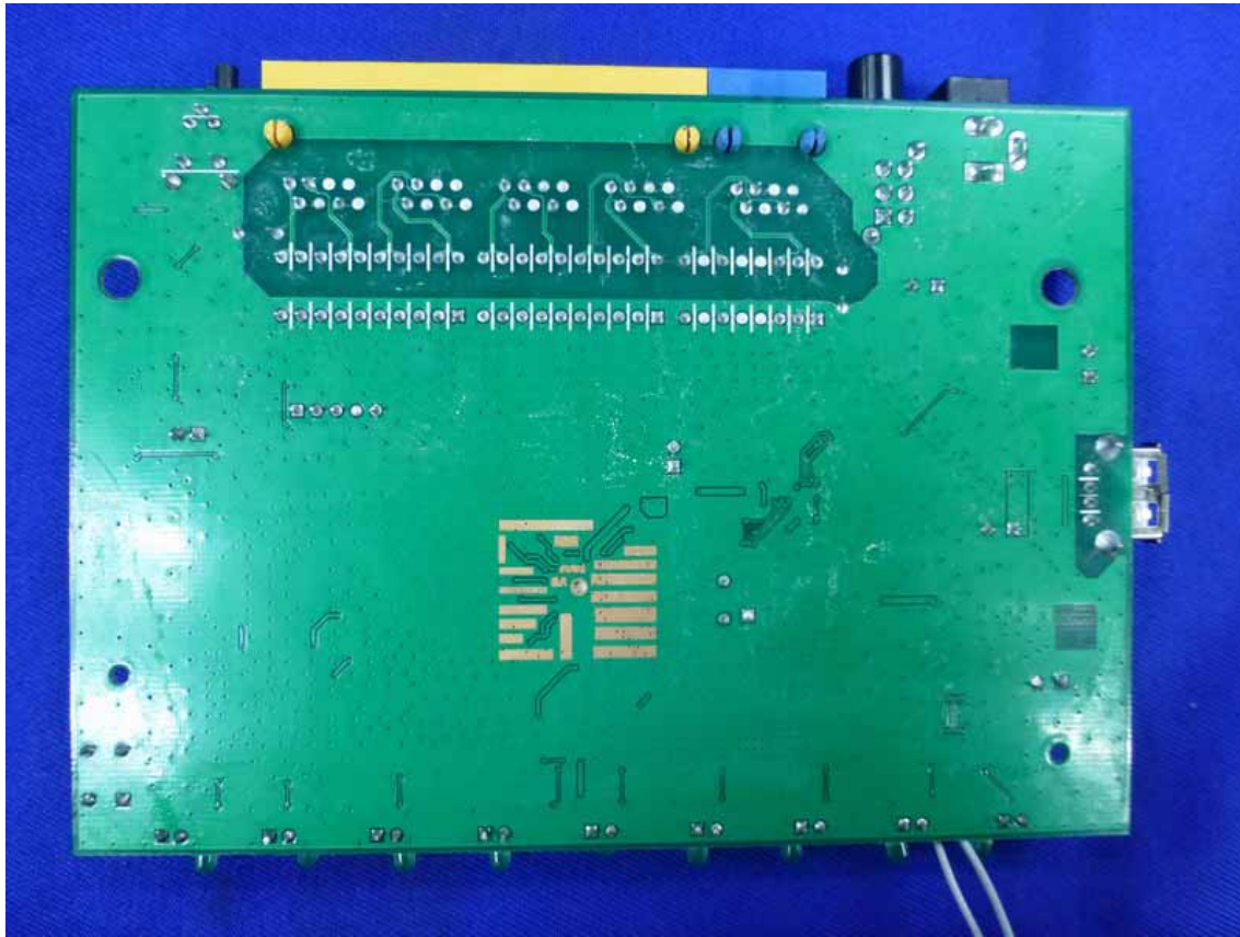
Figure 35 Backside of the PCB
