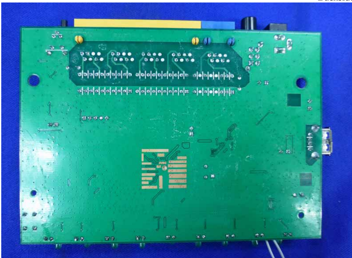
Figure 8 Backside of the PCB
