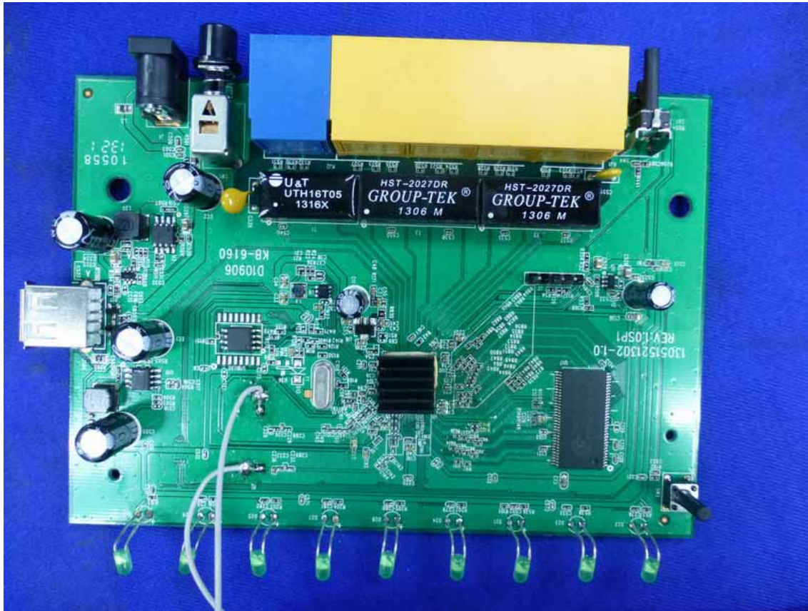
Figure 7 Frontside of the PCB
