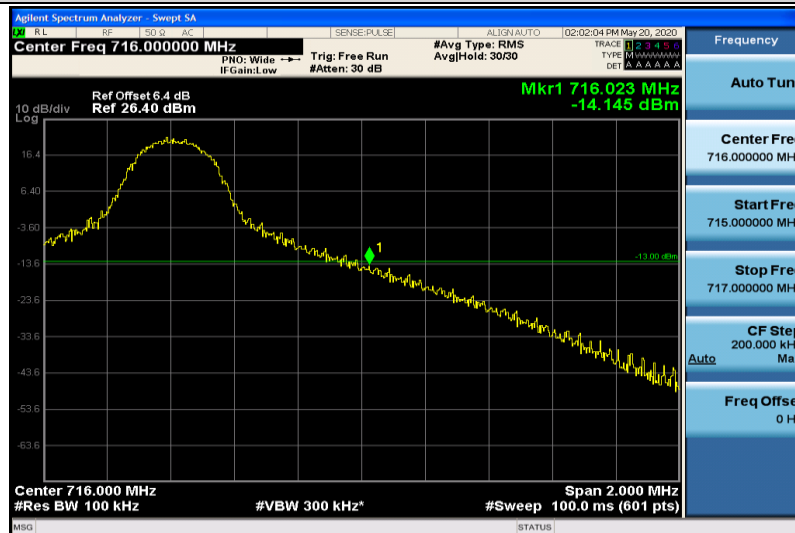
Band17-10MHz-16QAM-23800-1RB#49
