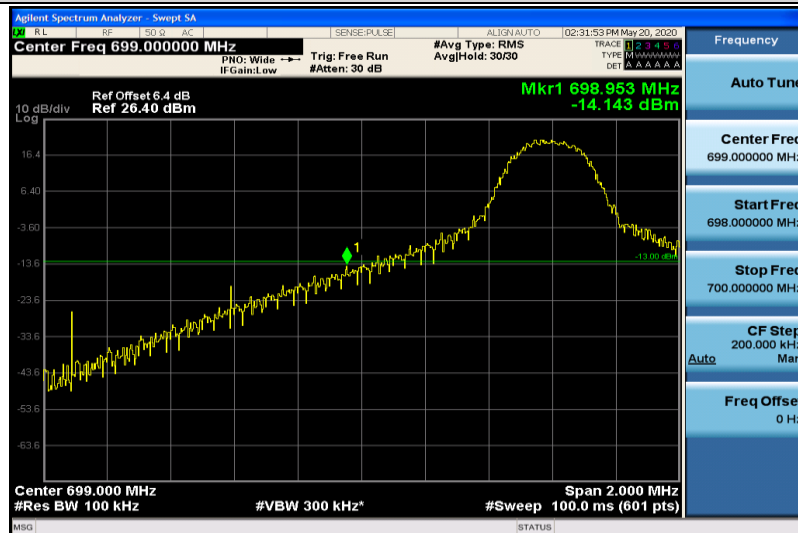
Band12-10MHz-16QAM-23060-1RB#0
