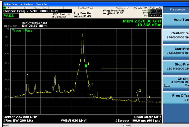
Band7-20MHz-16QAM-21350-1RB#99
