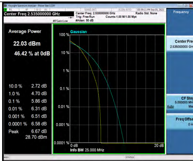
Band7-20MHz-16QAM-21100-27RB#0
