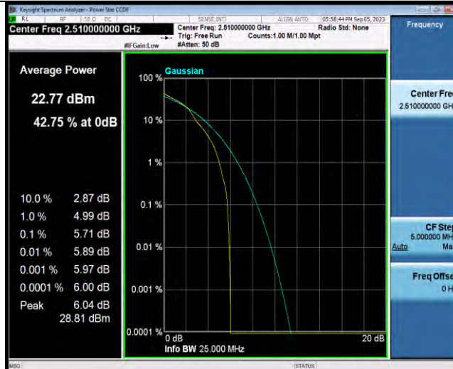
Band7-20MHz-16QAM-20850-27RB#0
