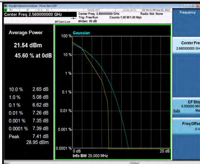
Band7-20MHz-16QAM-21350-27RB#0
