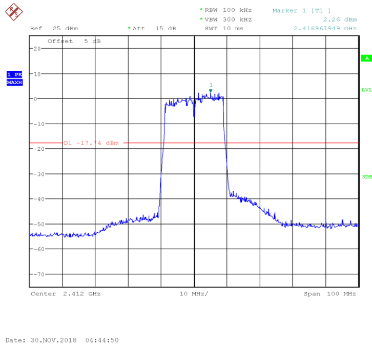
Fig 37. Conducted Spurious Emission (802.11n-20MHz, Ch1)
