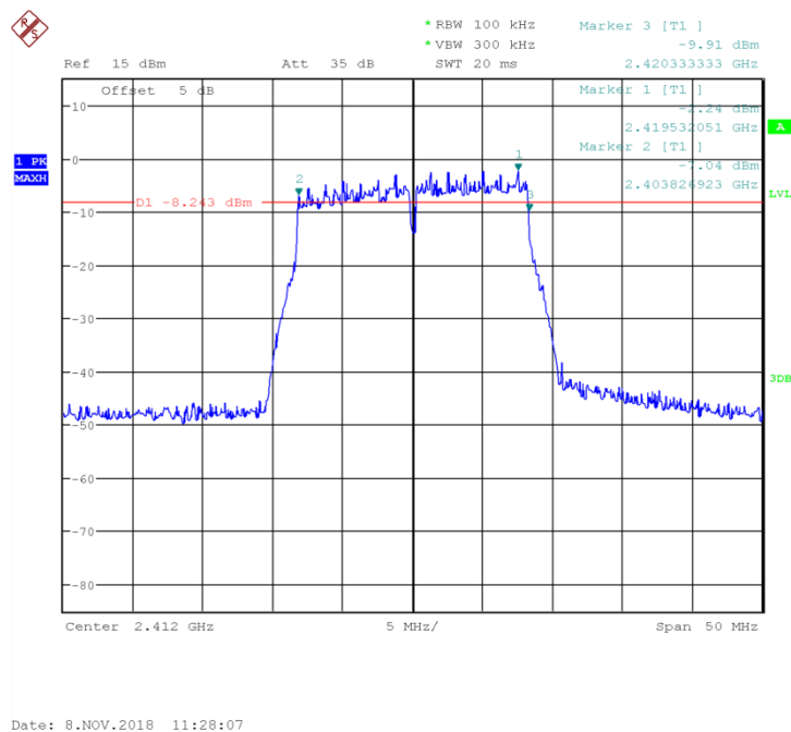
Fig 13. Occupied 6dB Bandwidth (802.11g, Ch1)
