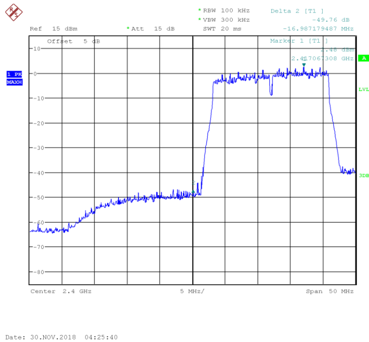
Fig 23. Band Edges (802.11n-20MHz, Ch1)
