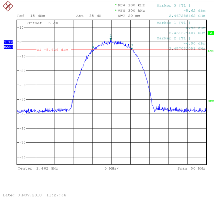
Fig 12. Occupied 6dB Bandwidth (802.11b, Ch11)
