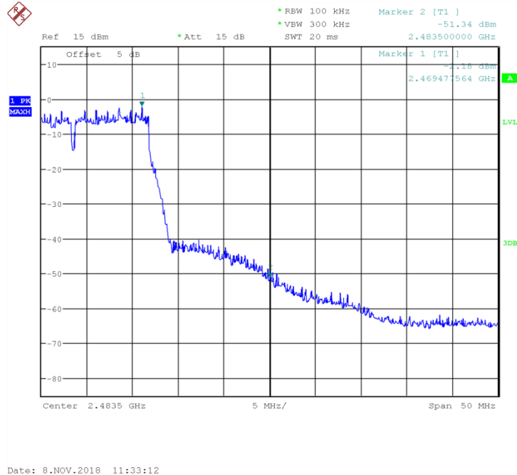
Fig 22. Band Edges (802.11g, Ch11)
