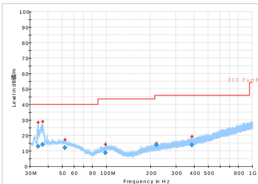
Fig 60. Radiated Spurious Emission (802.11b, Ch1,30MHz~1GHz)
