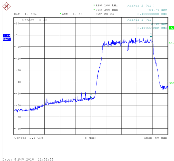
Fig 21. Band Edges (802.11g, Ch1)
