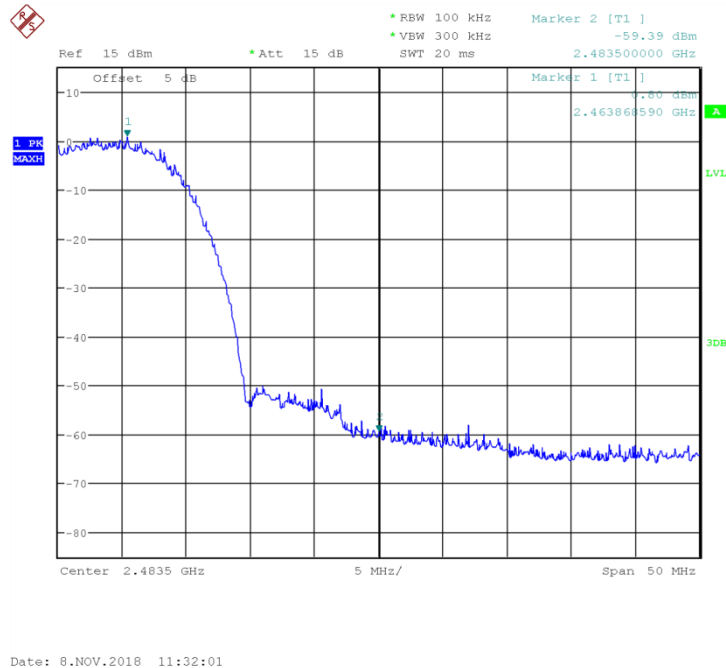
Fig 20. Band Edges (802.11b, Ch11)
