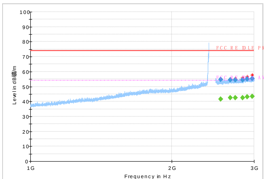
Fig 51. Radiated Spurious Emission (802.11g, Ch1,1GHz~3GHz)
