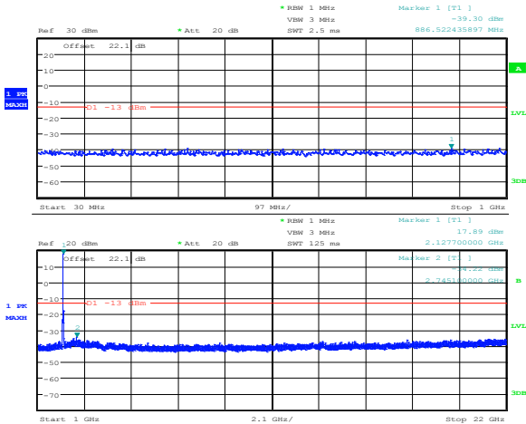
Figure 8.2-10: 15 MHz LTE QPSK 30 MHz – 22 GHz
