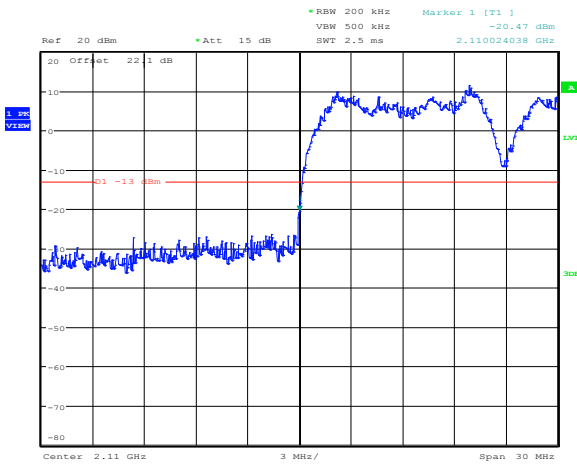
Figure 8.2-26: 10 MHz Lower Band edge QPSK
