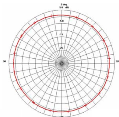
Azimuth 2.45 GHz
