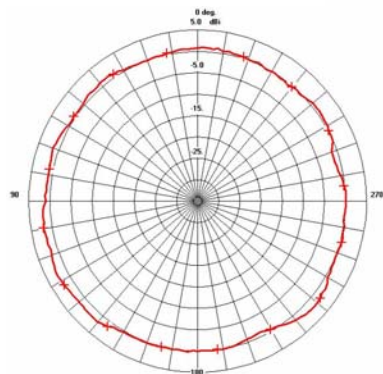
Azimuth 5.25 GHz
