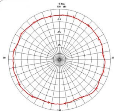
Azimuth 5.75 GHz
