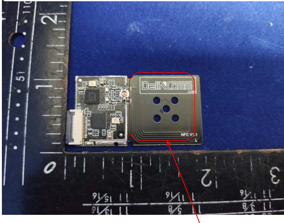
13.56MHz Antenna
