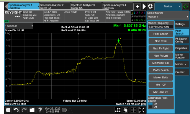
Channel 118 (5590MHz)
