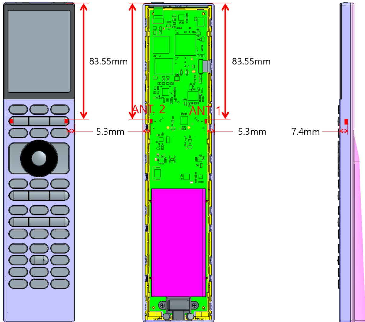
Figure E-1 Antenna Location (Front Side View)
