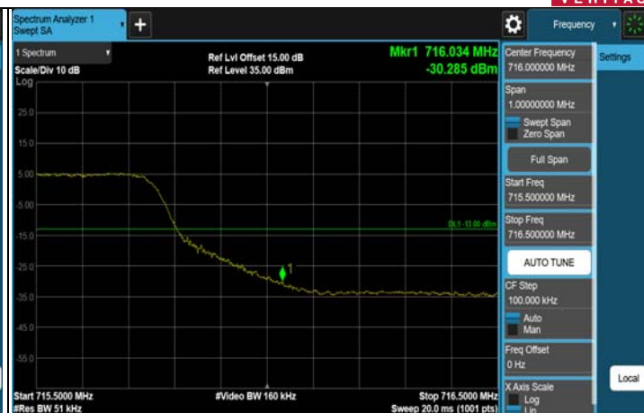
FULL CH 23825 (713.5 MHz)
