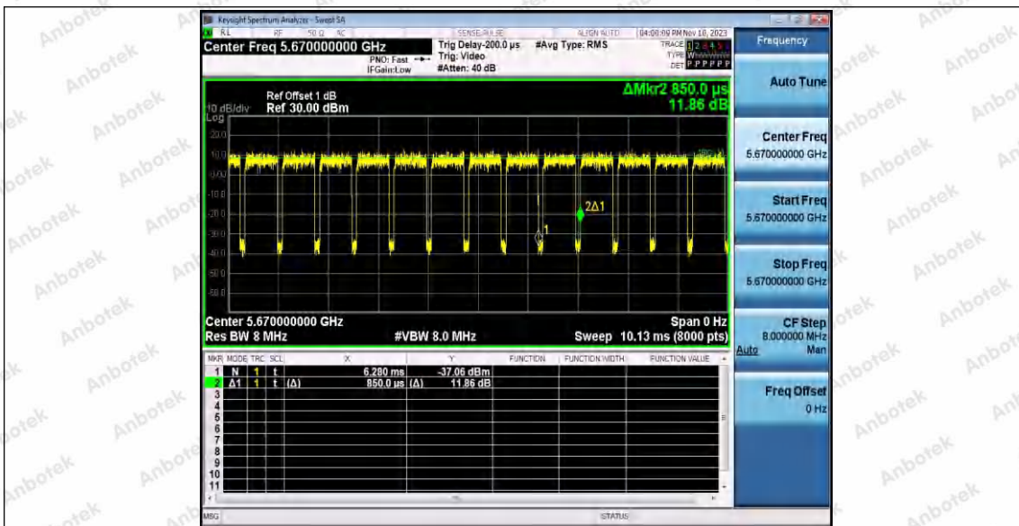
11AC40SISO_Ant2_5670
