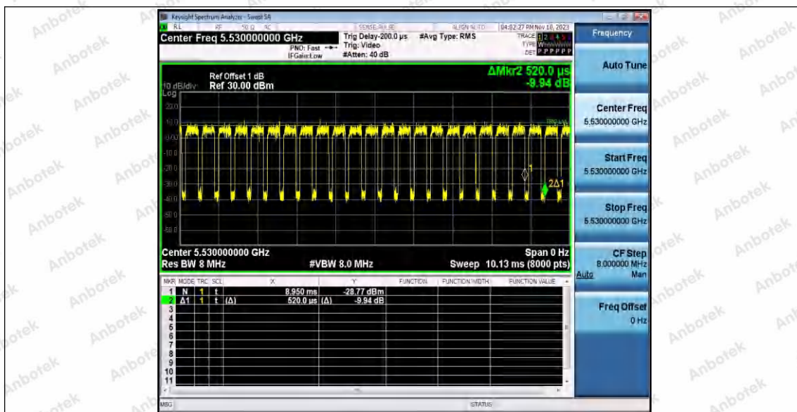
11AC80SISO_Ant2_5530
