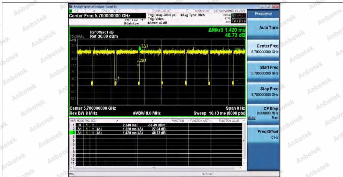
11AC20SISO_Ant2_5700
