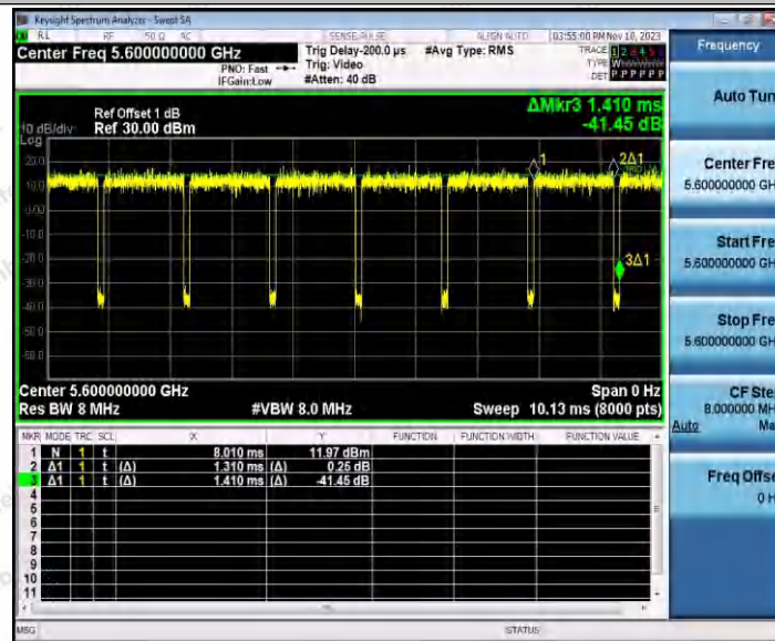
11AC20SISO_Ant2_5600
