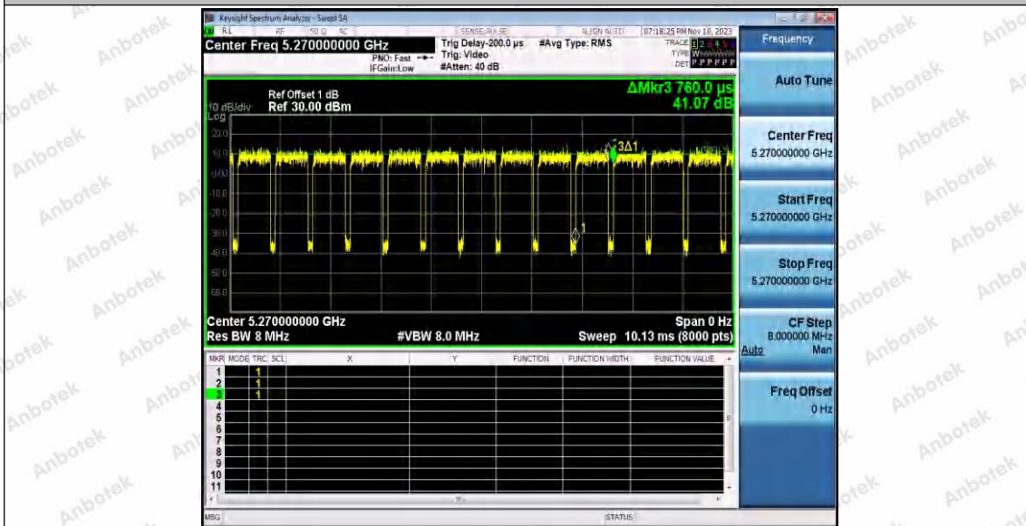
11AC40SISO_Ant1_5270
