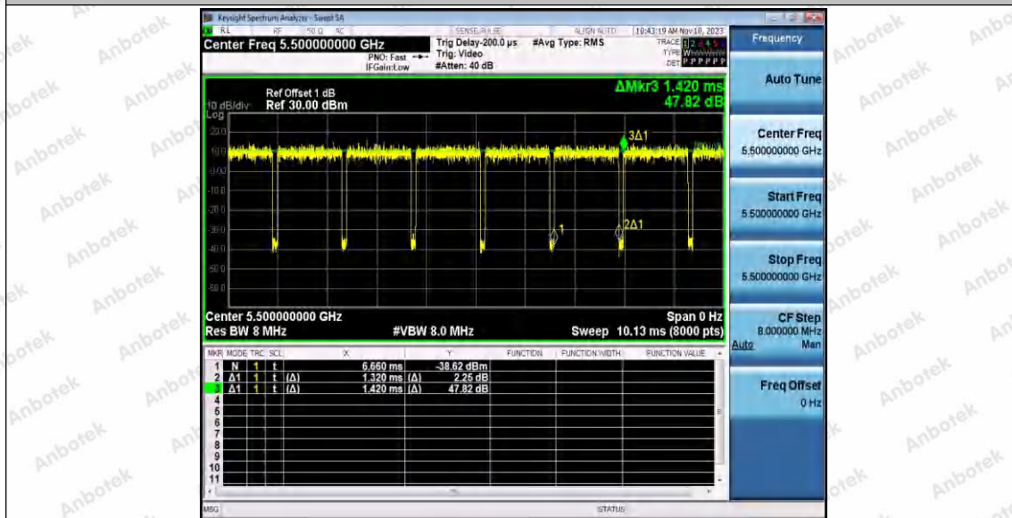
11AC20SISO_Ant2_5500
