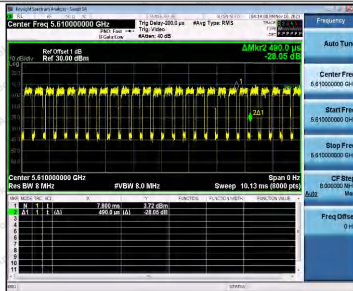
11AX80SISO_Ant2_5610
