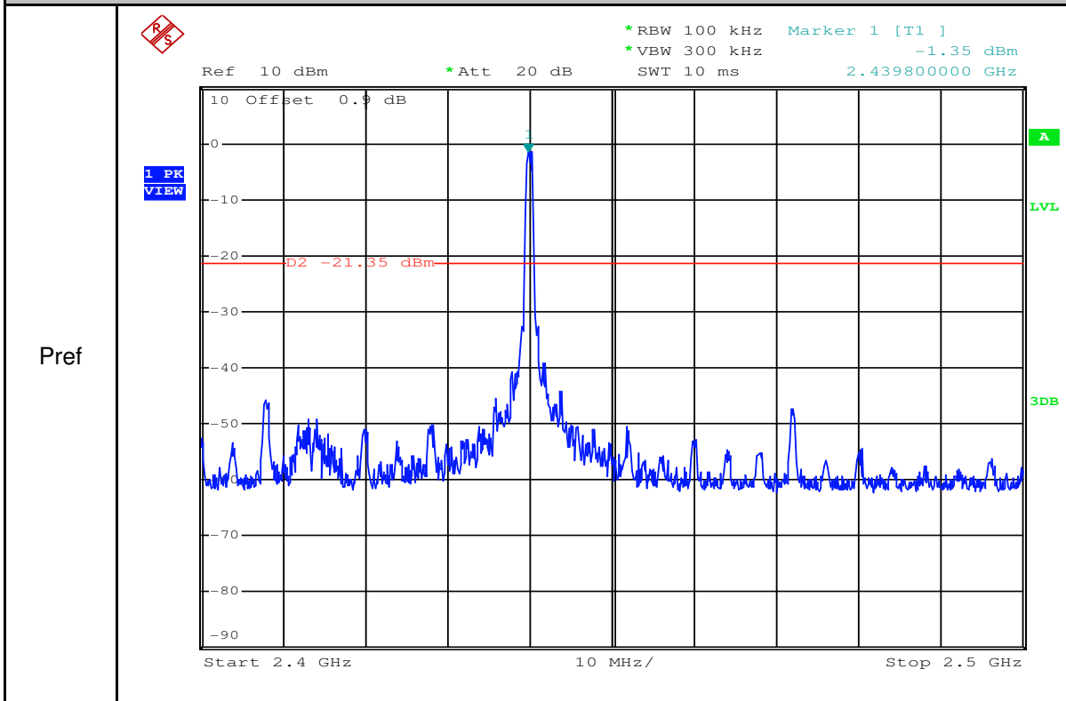
RF Conducted Spurious Emissions_BLE_2440_Ant1
