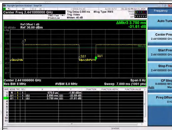
NTVN-2DH5-Ant1-2441
