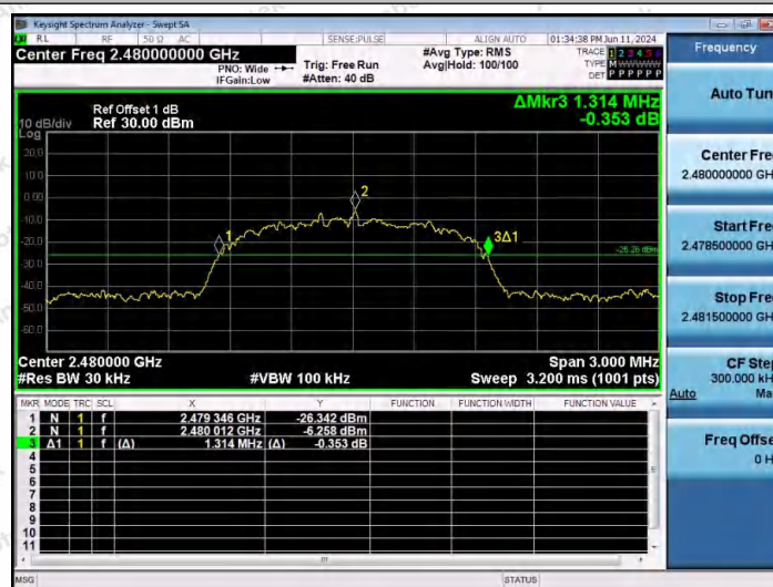
3DH5-Ant1-2480
