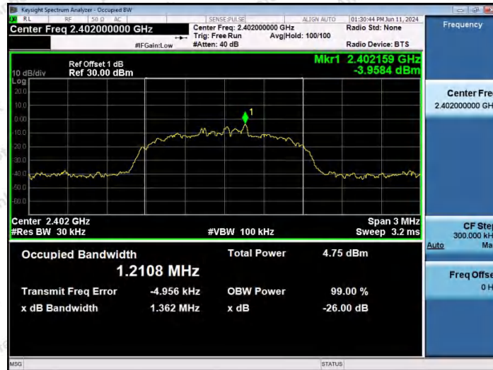
3DH5-Ant1-2402
