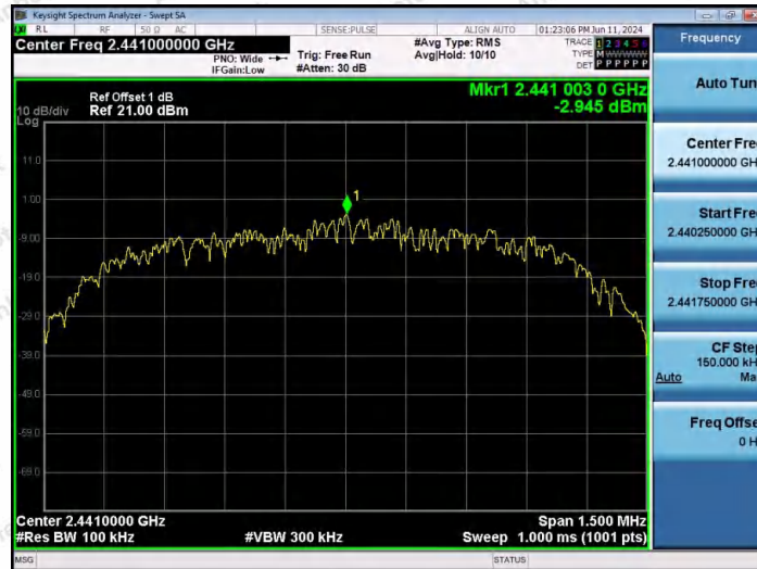
2DH5-Ant1-2441-0~Reference-PASS
