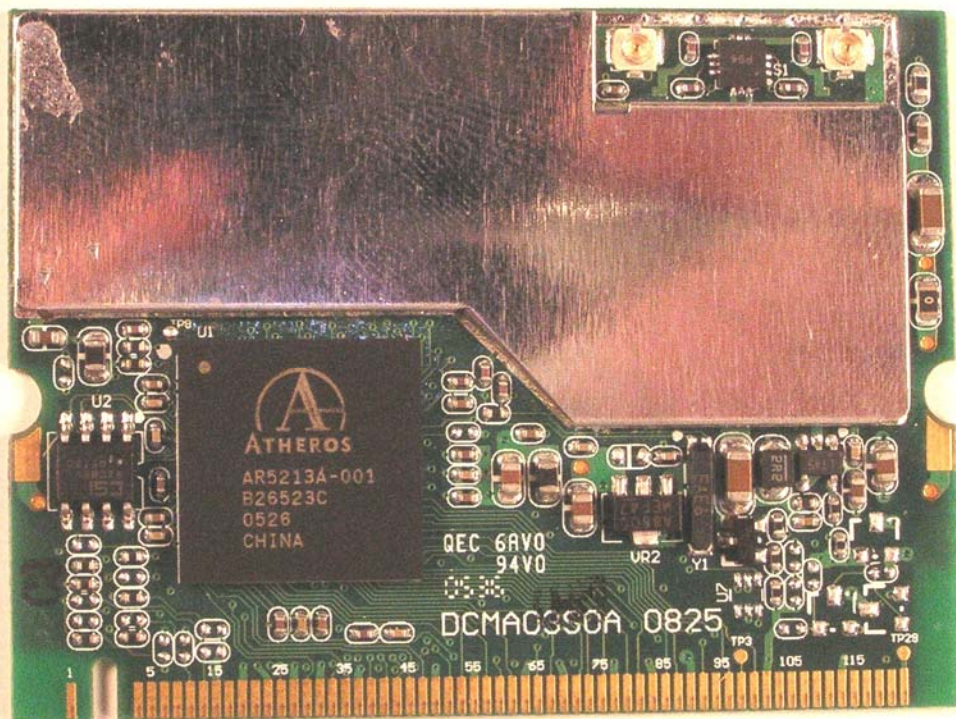
Top view of CM9-C1 with RF shielding installed
