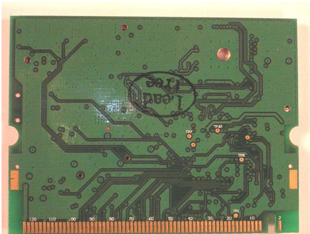
Bottom view of CM9-C1
