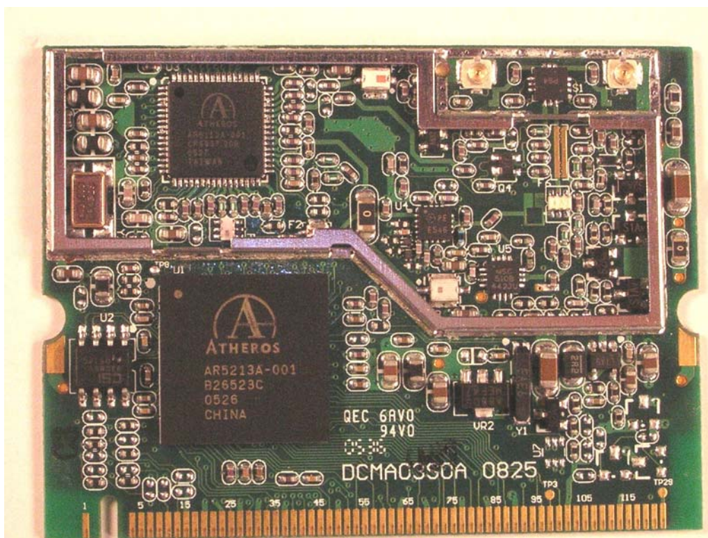
Top view of CM9-C1 with RF shielding removed
