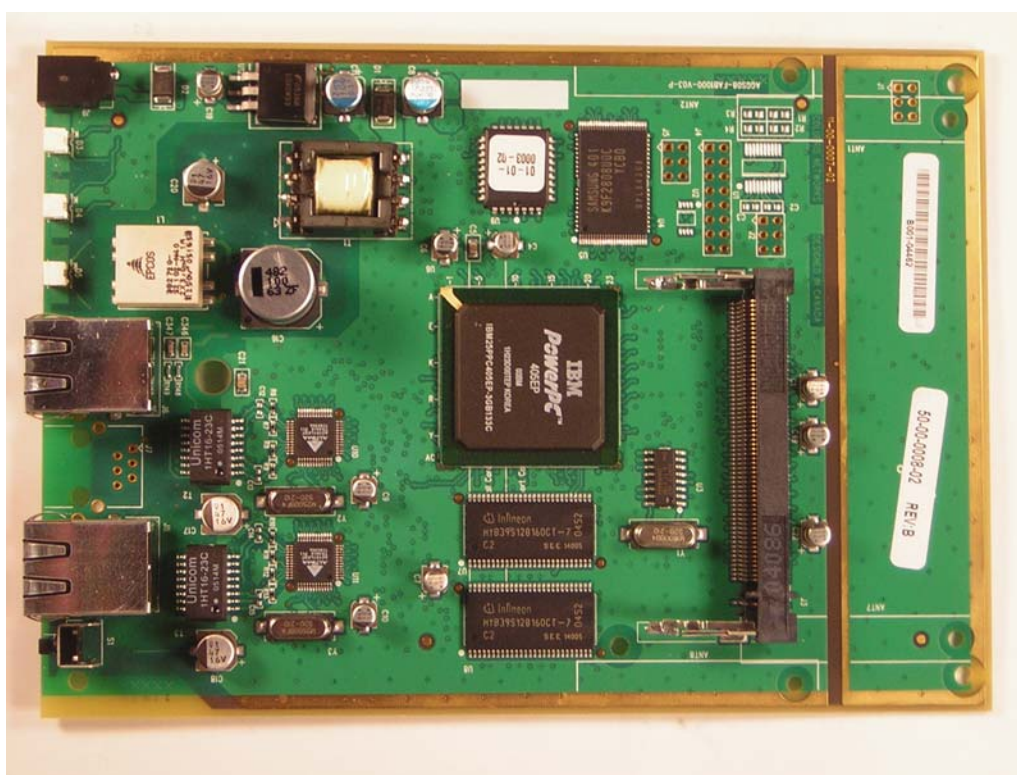
Top view of host board
