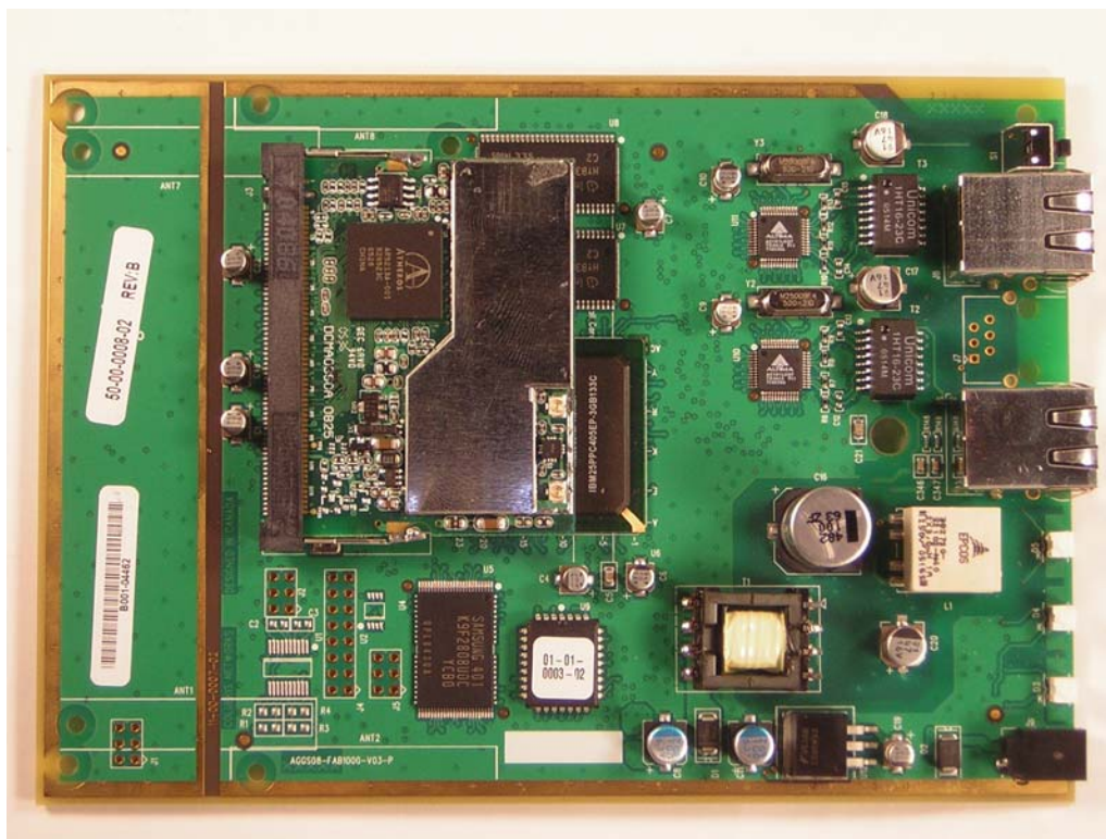
Top view of CM9-C1 installed on host board
