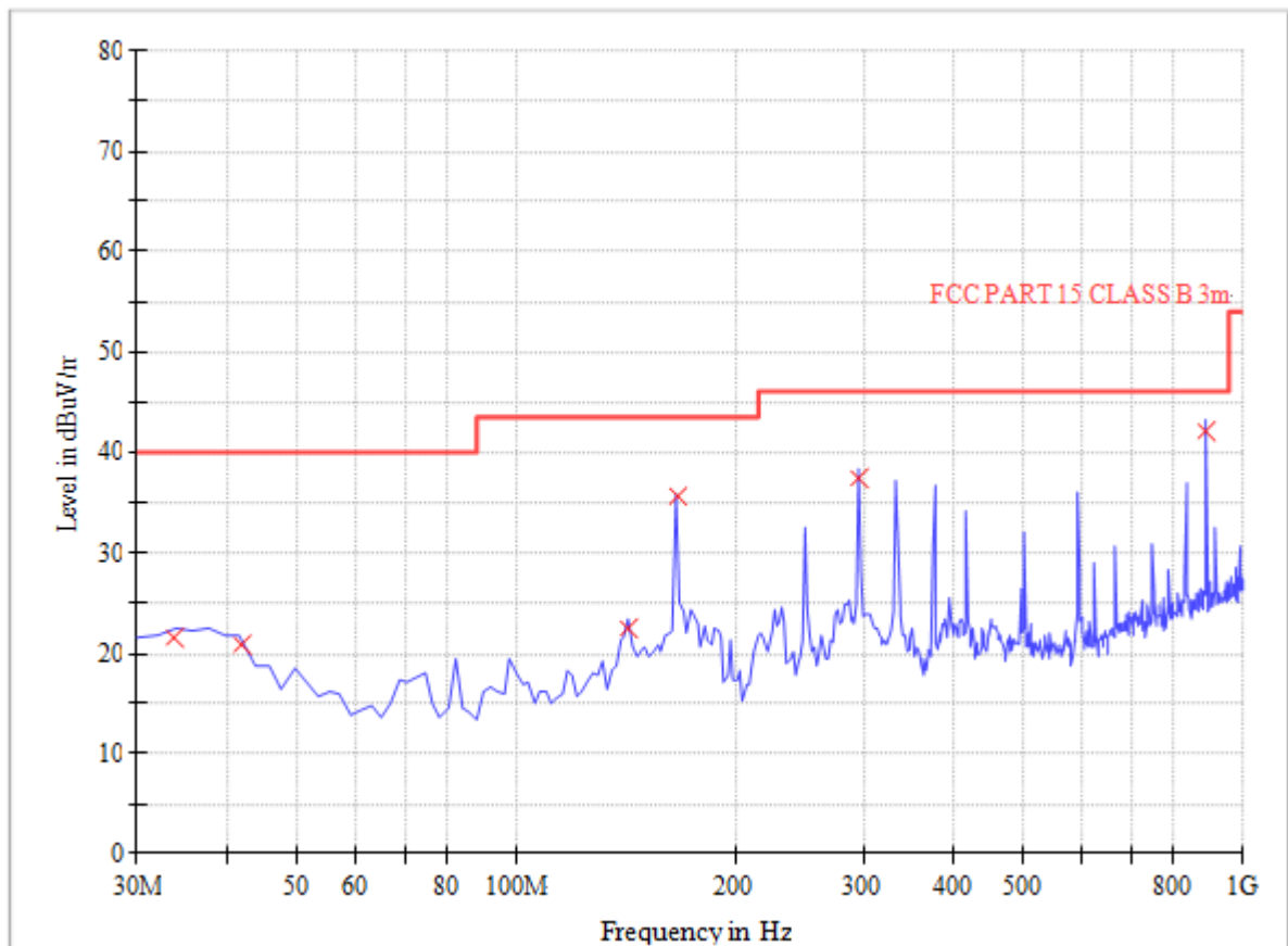
(Plot D: Test Antenna Horizontal 30M - 1G)
