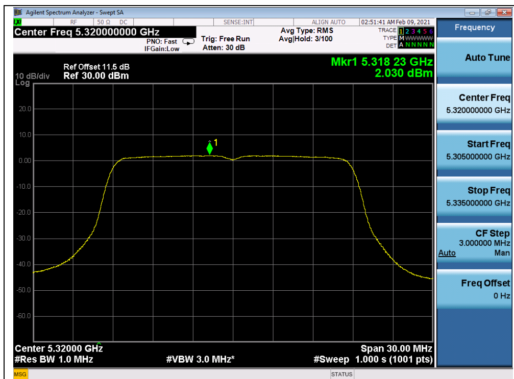
(Channel 64, 5320MHz, 802.11ac (VHT20), ANT0)
