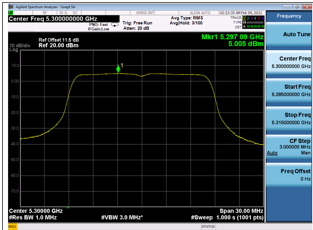
(Channel 60, 5300MHz, 802.11a, ANT0)
