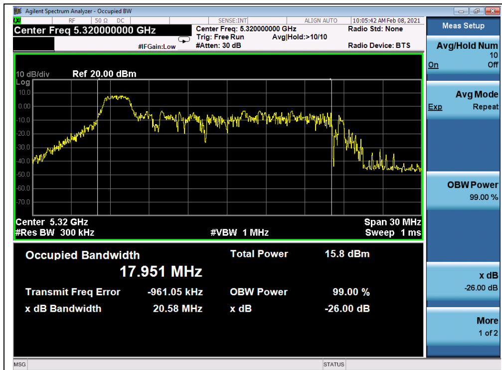
(Channel 64, 5320MHz, 802.11ax (HEW20)(RU26))
