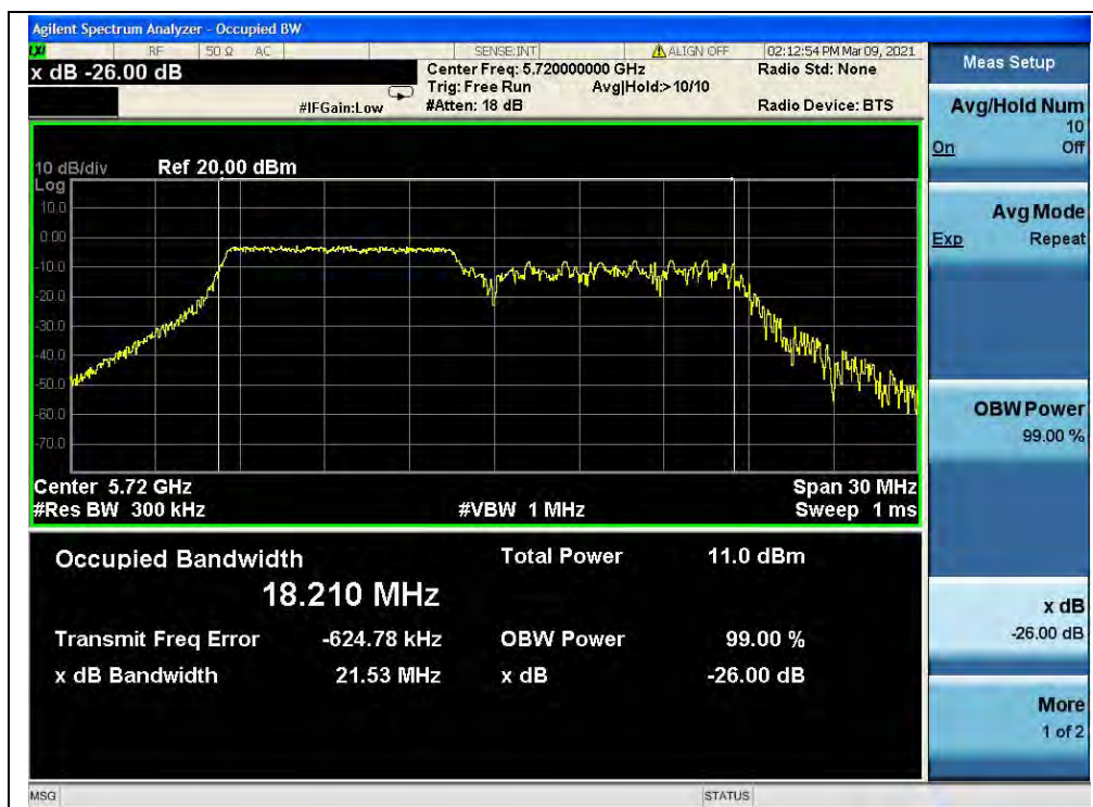
(Channel 144, 5720MHz, 802.11ax (HEW20)(RU106))
