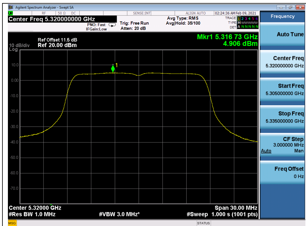
(Channel 64, 5320MHz, 802.11a, ANT0)
